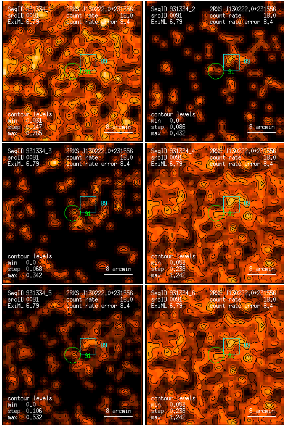
Figure 91: RASS 931334: detection 0091: band rate images, Gaussian filter: (1) PSPC channels 11 – 41, (2) 52 – 90, (3) 91 – 201, (4) 11 – 235, (5) 52 – 201, (6) 11 – 201. Broad band rates in counts/ks. Band rate contour levels in counts/ks/arcmin 2 .
