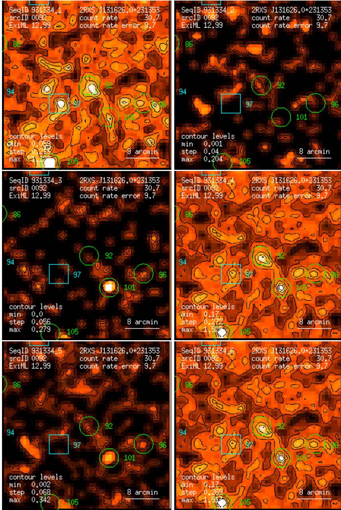
Figure 92: RASS 931334: detection 0092: band rate images, Gaussian filter: (1) PSPC channels 11 – 41, (2) 52 – 90, (3) 91 – 201, (4) 11 – 235, (5) 52 – 201, (6) 11 – 201. Broad band rates in counts/ks. Band rate contour levels in counts/ks/arcmin 2 .
