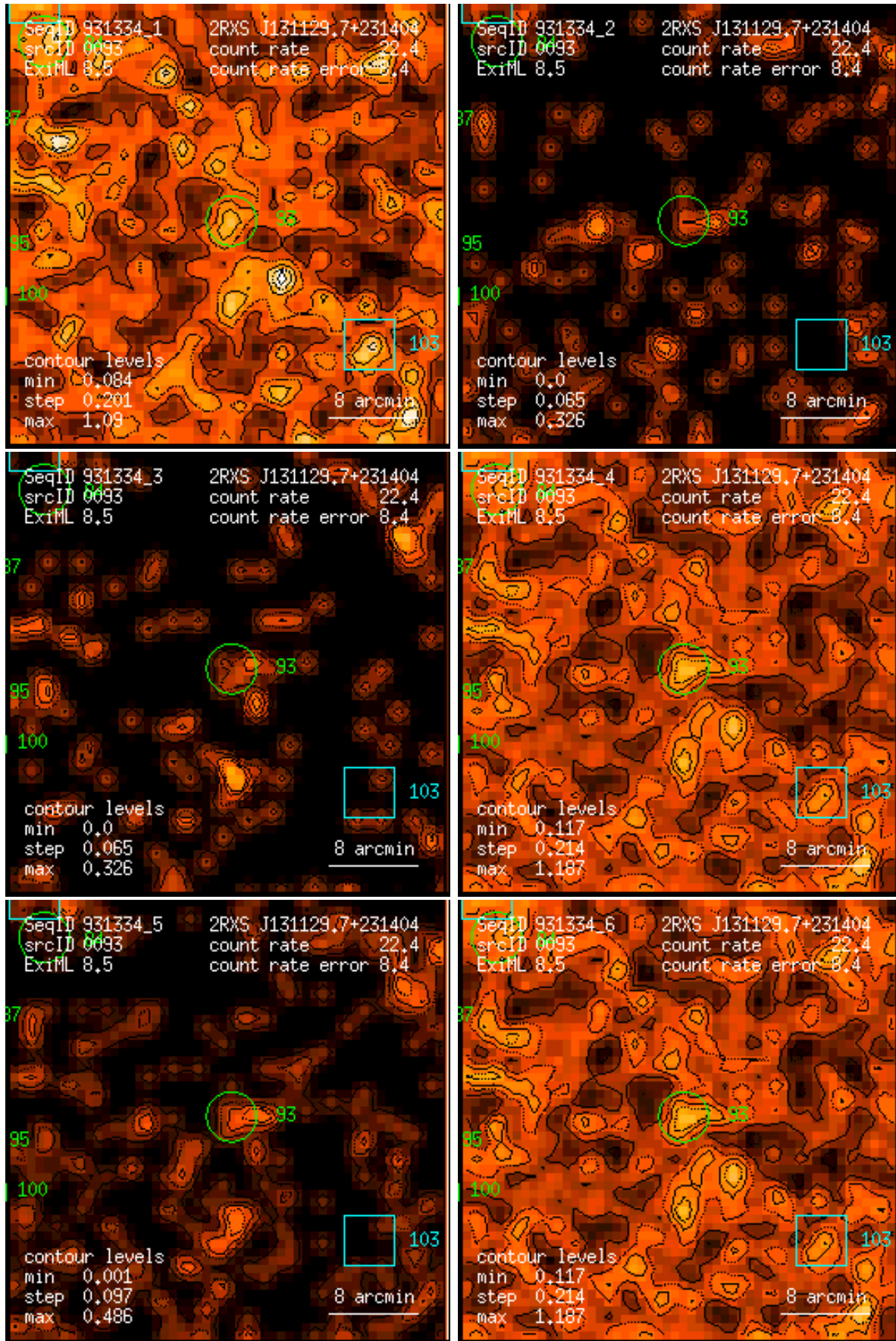
Figure 93: RASS 931334: detection 0093: band rate images, Gaussian filter: (1) PSPC channels 11 – 41, (2) 52 – 90, (3) 91 – 201, (4) 11 – 235, (5) 52 – 201, (6) 11 – 201. Broad band rates in counts/ks. Band rate contour levels in counts/ks/arcmin 2 .
