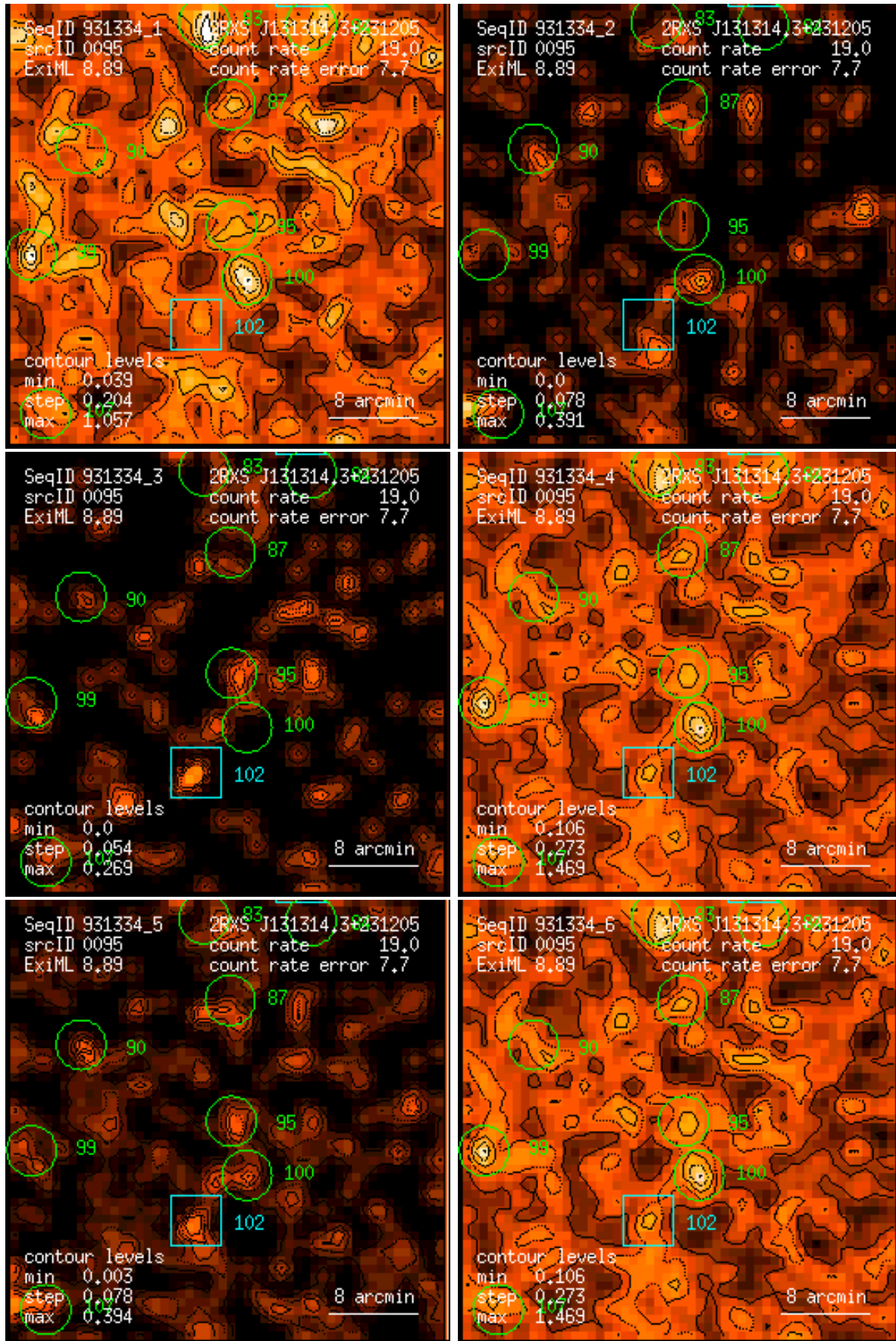
Figure 95: RASS 931334: detection 0095: band rate images, Gaussian filter: (1) PSPC channels 11 – 41, (2) 52 – 90, (3) 91 – 201, (4) 11 – 235, (5) 52 – 201, (6) 11 – 201. Broad band rates in counts/ks. Band rate contour levels in counts/ks/arcmin 2 .
