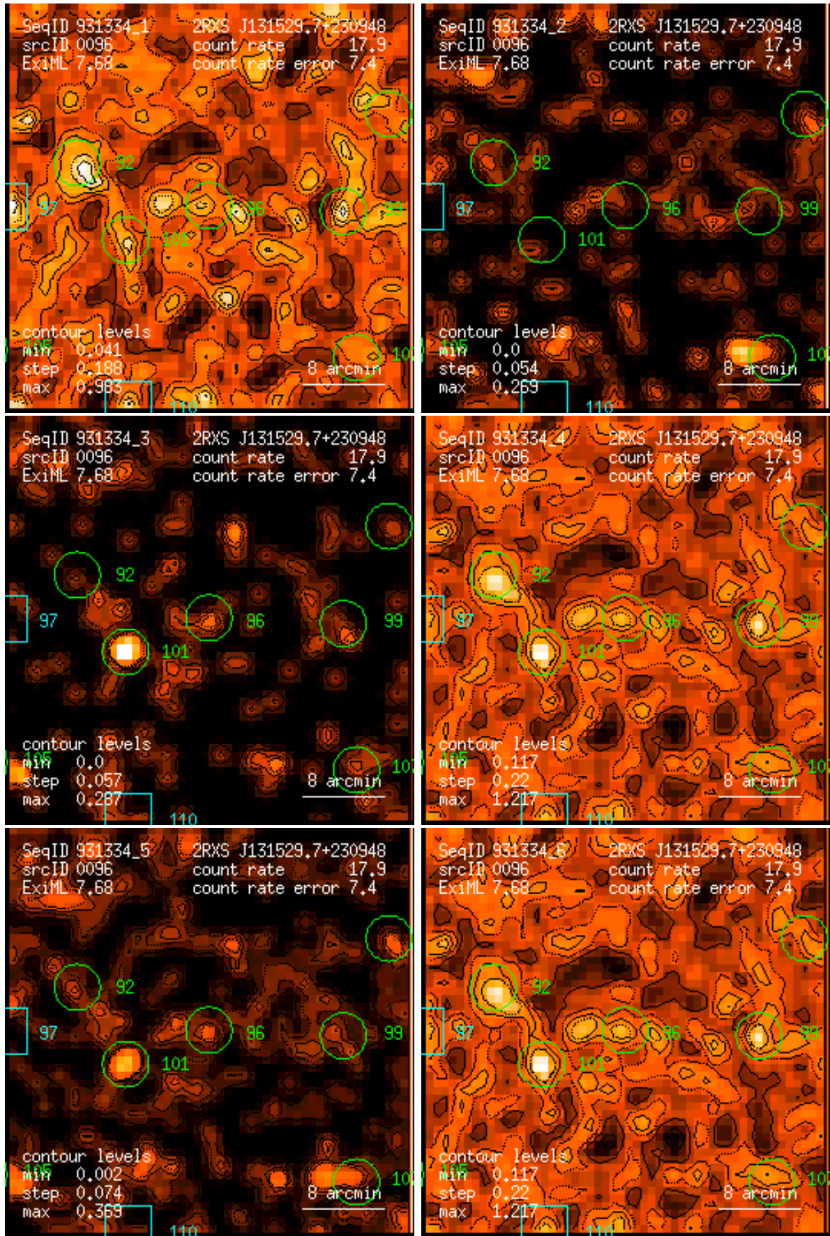
Figure 96: RASS 931334: detection 0096: band rate images, Gaussian filter: (1) PSPC channels 11 – 41, (2) 52 – 90, (3) 91 – 201, (4) 11 – 235, (5) 52 – 201, (6) 11 – 201. Broad band rates in counts/ks. Band rate contour levels in counts/ks/arcmin 2 .
