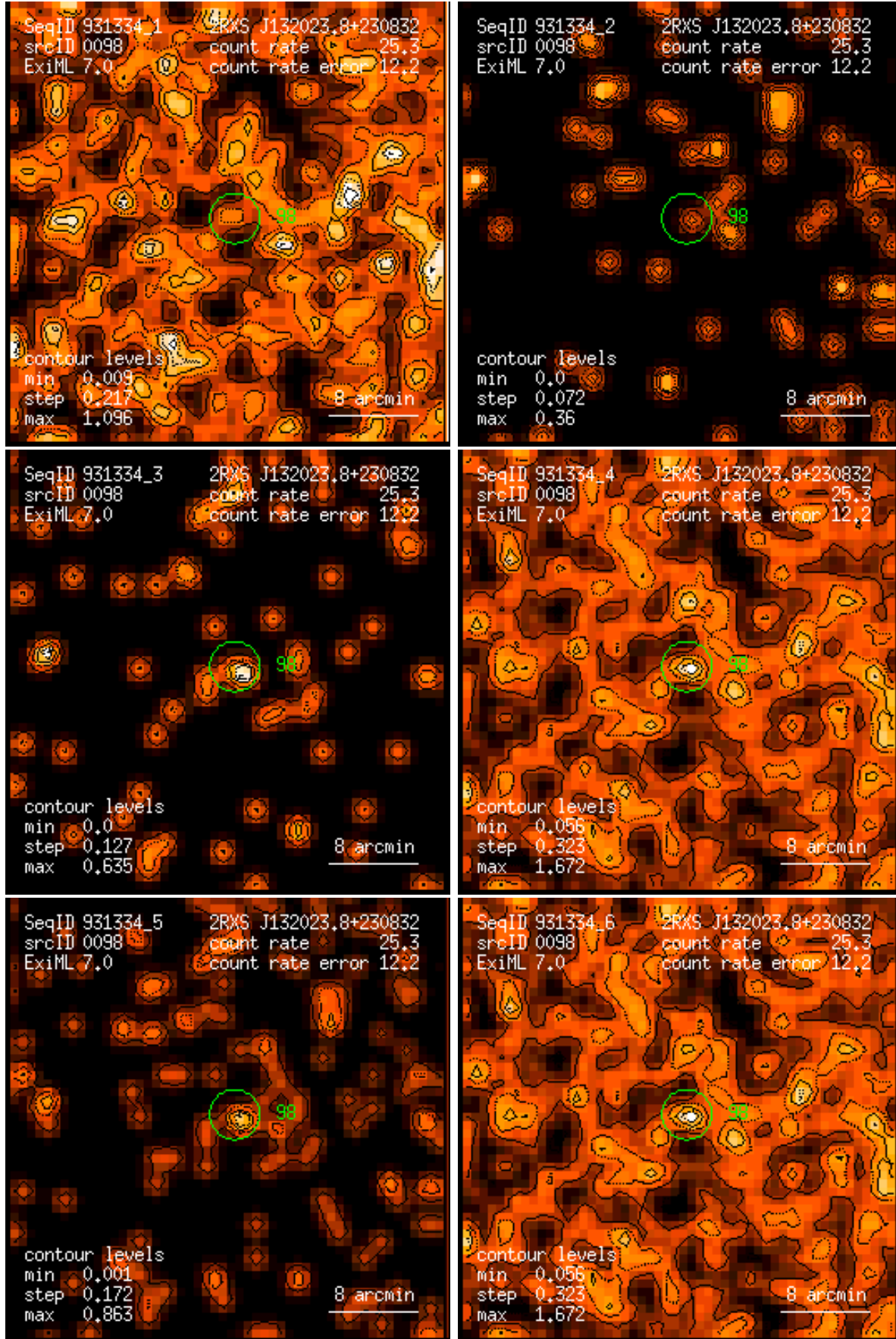
Figure 98: RASS 931334: detection 0098: band rate images, Gaussian filter: (1) PSPC channels 11 – 41, (2) 52 – 90, (3) 91 – 201, (4) 11 – 235, (5) 52 – 201, (6) 11 – 201. Broad band rates in counts/ks. Band rate contour levels in counts/ks/arcmin 2 .
