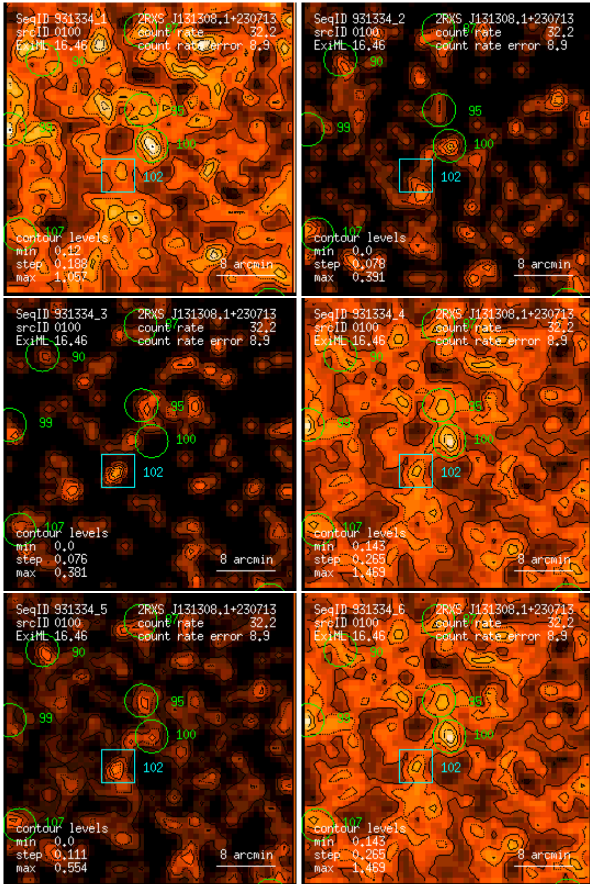
Figure 100: RASS 931334: detection 0100: band rate images, Gaussian filter: (1) PSPC channels 11 – 41, (2) 52 – 90, (3) 91 – 201, (4) 11 – 235, (5) 52 – 201, (6) 11 – 201. Broad band rates in counts/ks. Band rate contour levels in counts/ks/arcmin 2 .
