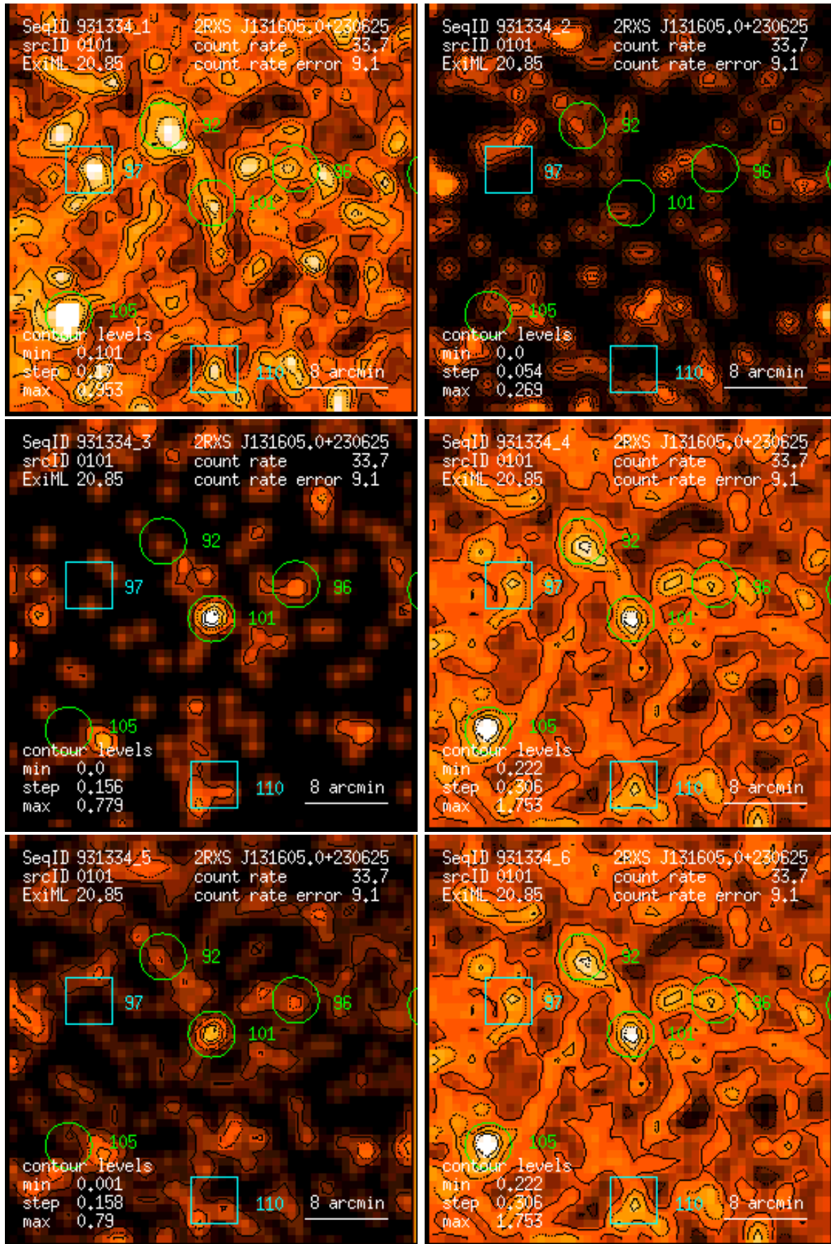
Figure 101: RASS 931334: detection 0101: band rate images, Gaussian filter: (1) PSPC channels 11 – 41, (2) 52 – 90, (3) 91 – 201, (4) 11 – 235, (5) 52 – 201, (6) 11 – 201. Broad band rates in counts/ks. Band rate contour levels in counts/ks/arcmin 2 .
