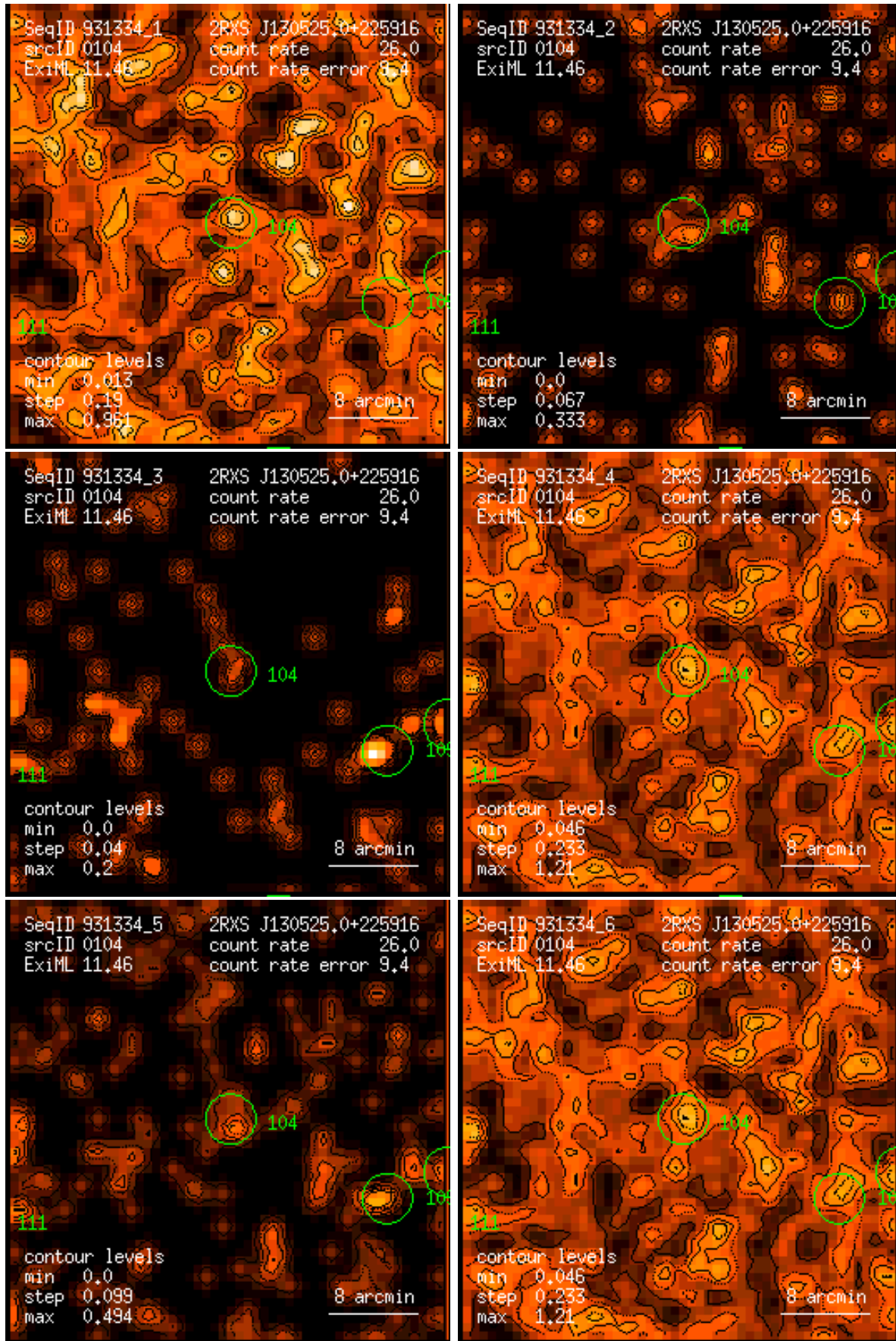
Figure 104: RASS 931334: detection 0104: band rate images, Gaussian filter: (1) PSPC channels 11 – 41, (2) 52 – 90, (3) 91 – 201, (4) 11 – 235, (5) 52 – 201, (6) 11 – 201. Broad band rates in counts/ks. Band rate contour levels in counts/ks/arcmin 2 .
