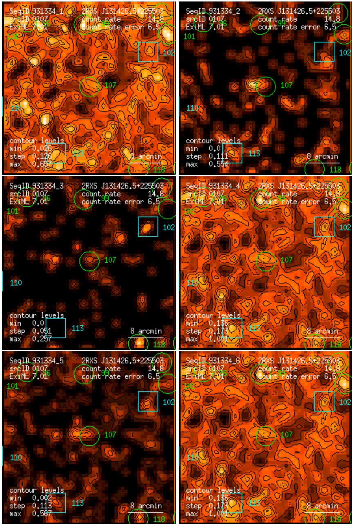
Figure 107: RASS 931334: detection 0107: band rate images, Gaussian filter: (1) PSPC channels 11 – 41, (2) 52 – 90, (3) 91 – 201, (4) 11 – 235, (5) 52 – 201, (6) 11 – 201. Broad band rates in counts/ks. Band rate contour levels in counts/ks/arcmin 2 .
