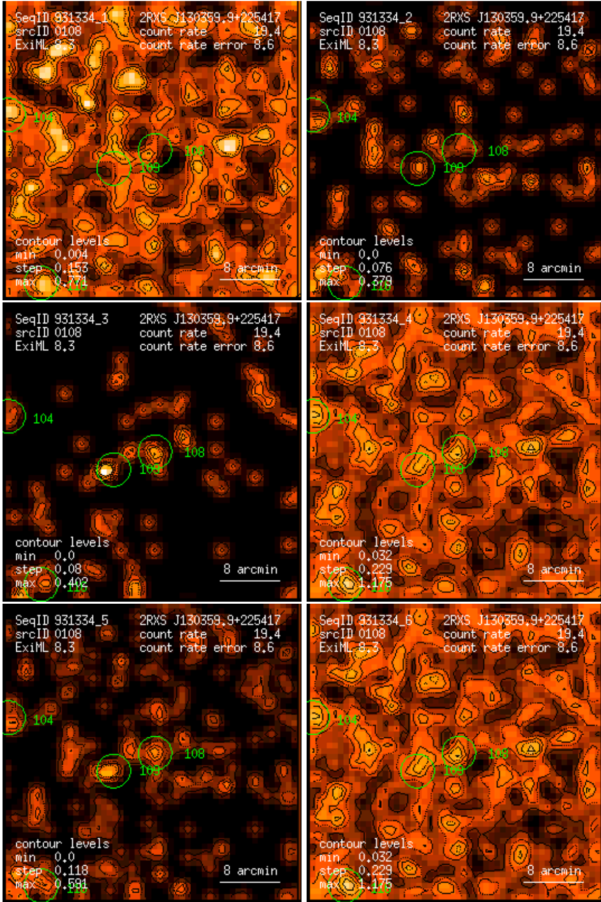
Figure 108: RASS 931334: detection 0108: band rate images, Gaussian filter: (1) PSPC channels 11 – 41, (2) 52 – 90, (3) 91 – 201, (4) 11 – 235, (5) 52 – 201, (6) 11 – 201. Broad band rates in counts/ks. Band rate contour levels in counts/ks/arcmin 2 .
