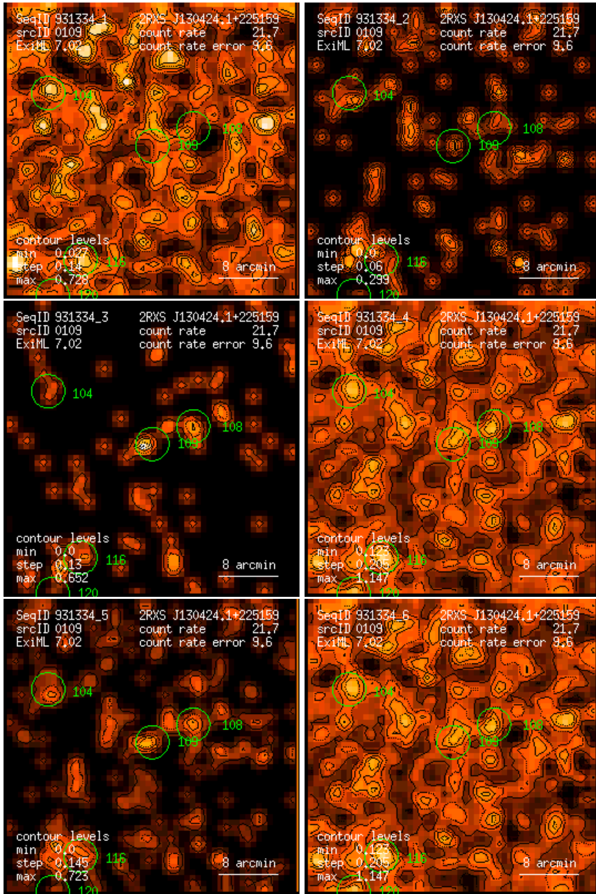
Figure 109: RASS 931334: detection 0109: band rate images, Gaussian filter: (1) PSPC channels 11 – 41, (2) 52 – 90, (3) 91 – 201, (4) 11 – 235, (5) 52 – 201, (6) 11 – 201. Broad band rates in counts/ks. Band rate contour levels in counts/ks/arcmin 2 .
