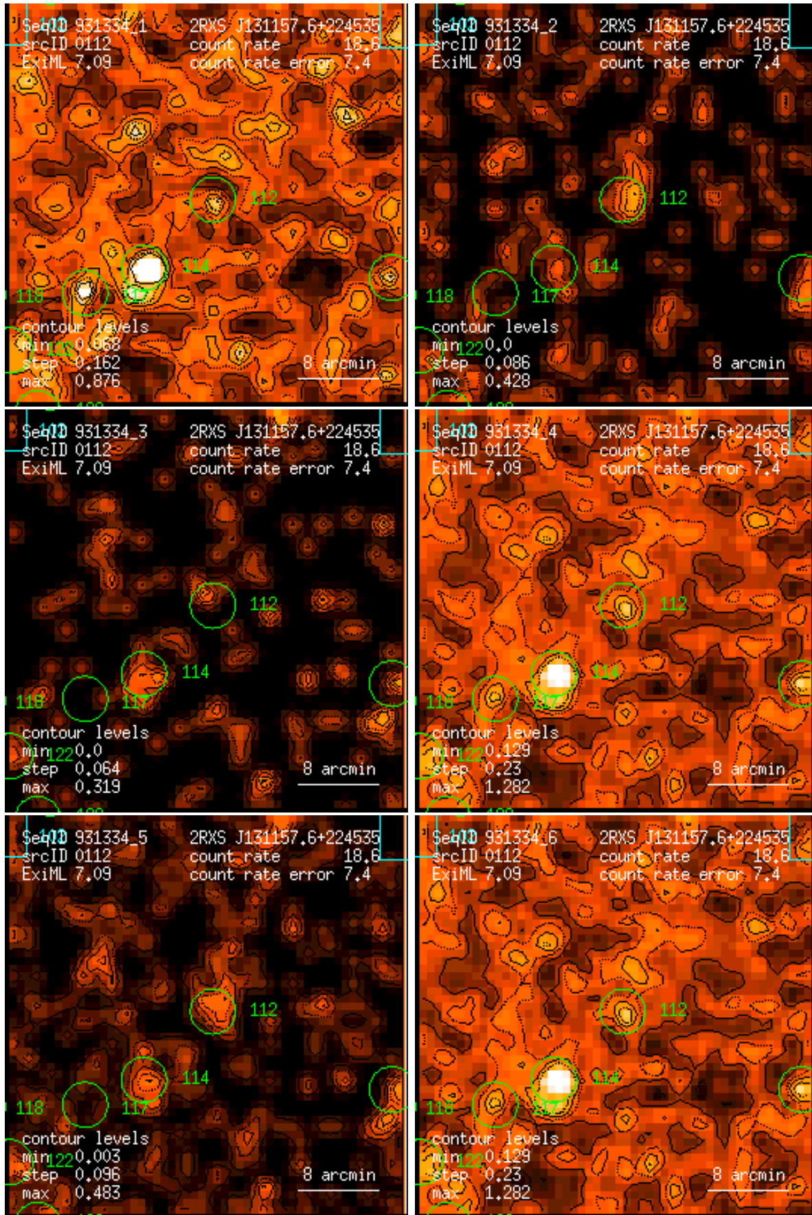
Figure 112: RASS 931334: detection 0112: band rate images, Gaussian filter: (1) PSPC channels 11 – 41, (2) 52 – 90, (3) 91 – 201, (4) 11 – 235, (5) 52 – 201, (6) 11 – 201. Broad band rates in counts/ks. Band rate contour levels in counts/ks/arcmin 2 .
