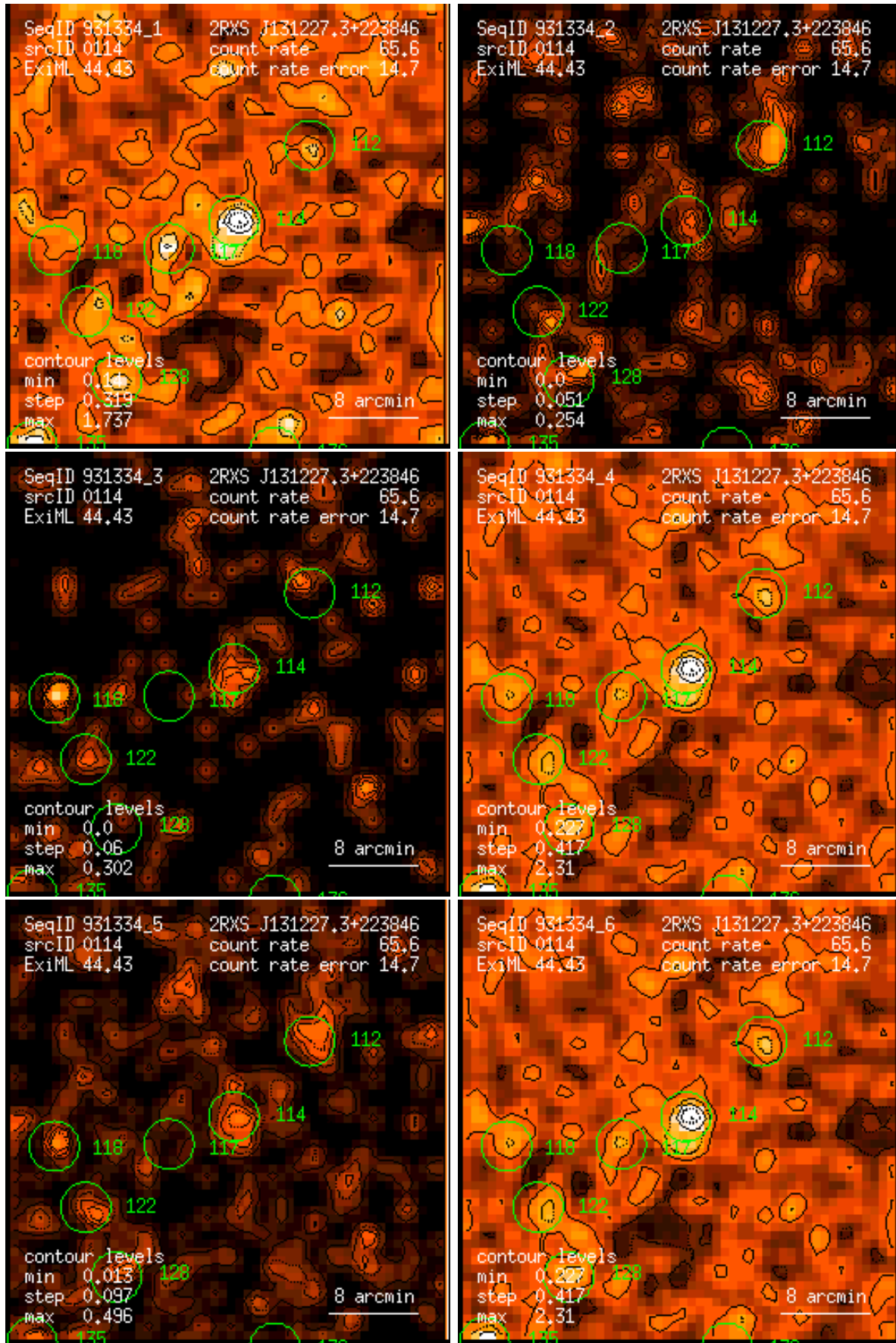
Figure 114: RASS 931334: detection 0114: band rate images, Gaussian filter: (1) PSPC channels 11 – 41, (2) 52 – 90, (3) 91 – 201, (4) 11 – 235, (5) 52 – 201, (6) 11 – 201. Broad band rates in counts/ks. Band rate contour levels in counts/ks/arcmin 2 .
