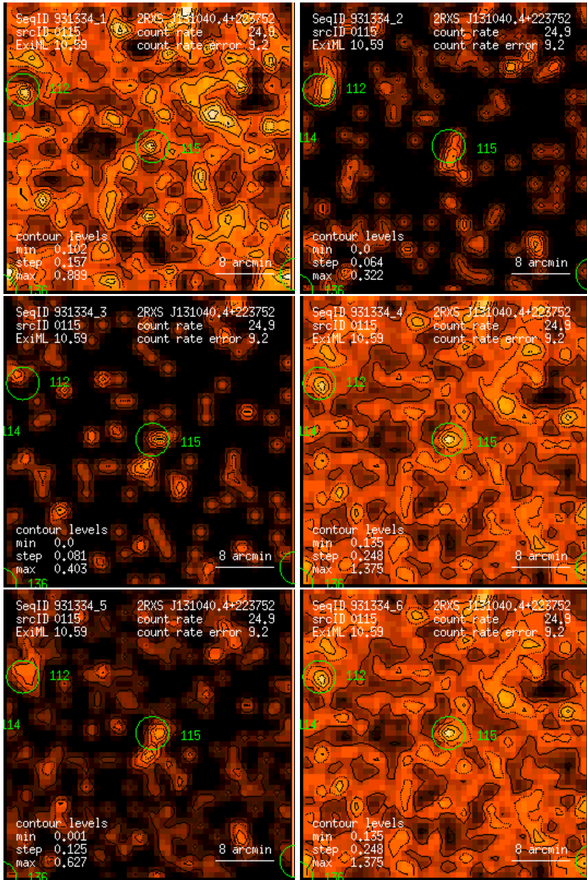
Figure 115: RASS 931334: detection 0115: band rate images, Gaussian filter: (1) PSPC channels 11 – 41, (2) 52 – 90, (3) 91 – 201, (4) 11 – 235, (5) 52 – 201, (6) 11 – 201. Broad band rates in counts/ks. Band rate contour levels in counts/ks/arcmin 2 .
