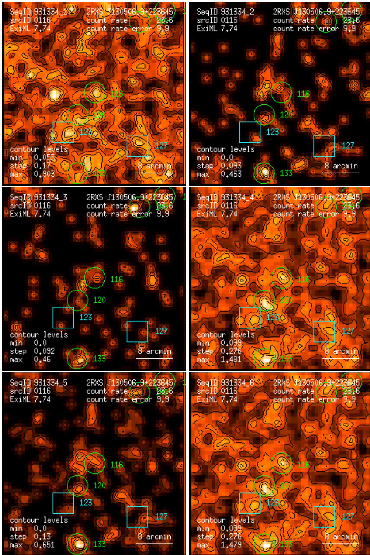
Figure 116: RASS 931334: detection 0116: band rate images, Gaussian filter: (1) PSPC channels 11 – 41, (2) 52 – 90, (3) 91 – 201, (4) 11 – 235, (5) 52 – 201, (6) 11 – 201. Broad band rates in counts/ks. Band rate contour levels in counts/ks/arcmin 2 .
