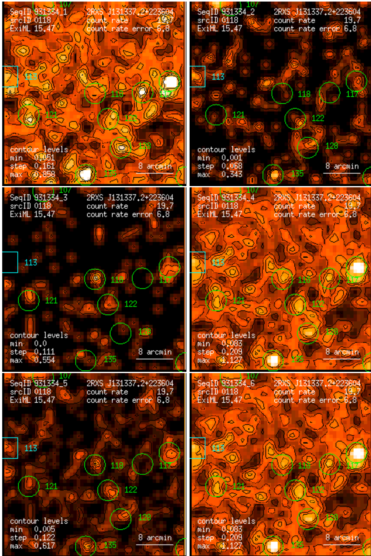
Figure 118: RASS 931334: detection 0118: band rate images, Gaussian filter: (1) PSPC channels 11 – 41, (2) 52 – 90, (3) 91 – 201, (4) 11 – 235, (5) 52 – 201, (6) 11 – 201. Broad band rates in counts/ks. Band rate contour levels in counts/ks/arcmin 2 .
