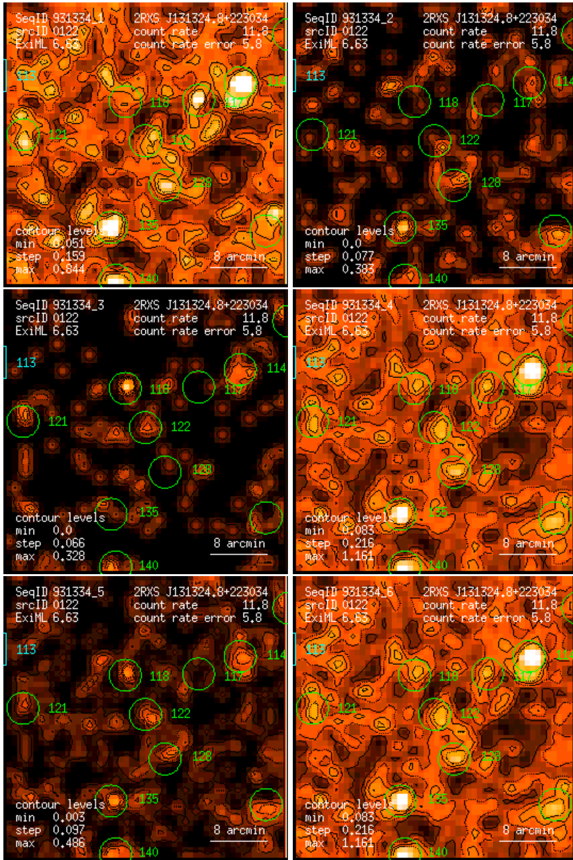
Figure 122: RASS 931334: detection 0122: band rate images, Gaussian filter: (1) PSPC channels 11 – 41, (2) 52 – 90, (3) 91 – 201, (4) 11 – 235, (5) 52 – 201, (6) 11 – 201. Broad band rates in counts/ks. Band rate contour levels in counts/ks/arcmin 2 .
