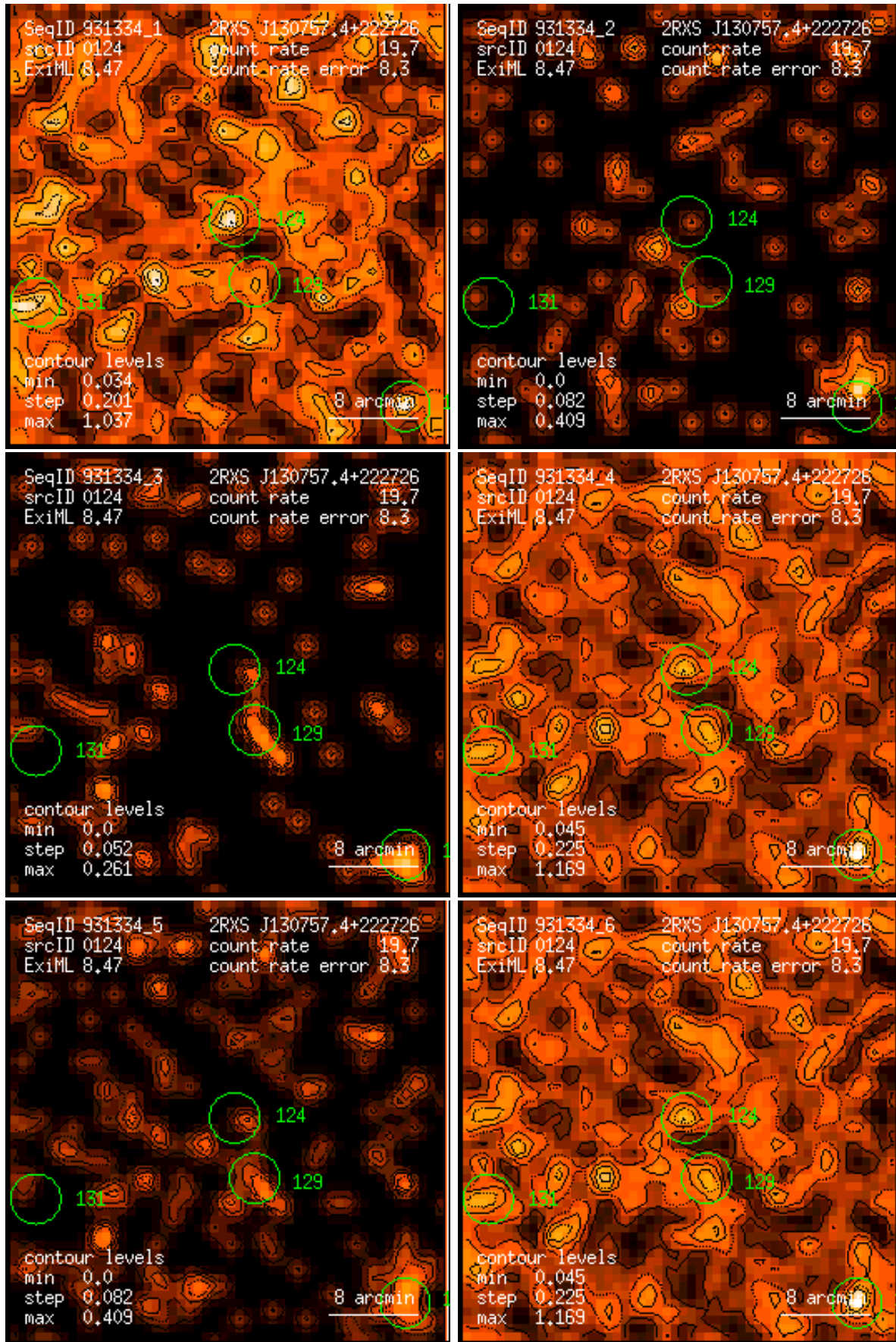
Figure 124: RASS 931334: detection 0124: band rate images, Gaussian filter: (1) PSPC channels 11 – 41, (2) 52 – 90, (3) 91 – 201, (4) 11 – 235, (5) 52 – 201, (6) 11 – 201. Broad band rates in counts/ks. Band rate contour levels in counts/ks/arcmin 2 .
