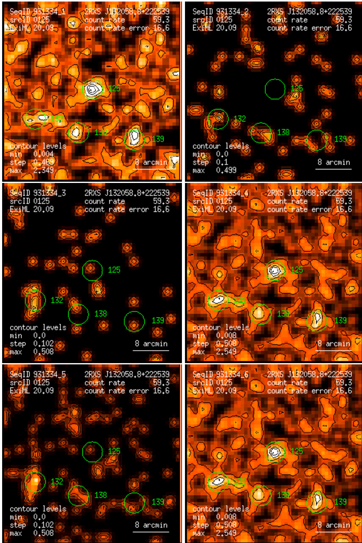
Figure 125: RASS 931334: detection 0125: band rate images, Gaussian filter: (1) PSPC channels 11 – 41, (2) 52 – 90, (3) 91 – 201, (4) 11 – 235, (5) 52 – 201, (6) 11 – 201. Broad band rates in counts/ks. Band rate contour levels in counts/ks/arcmin 2 .
