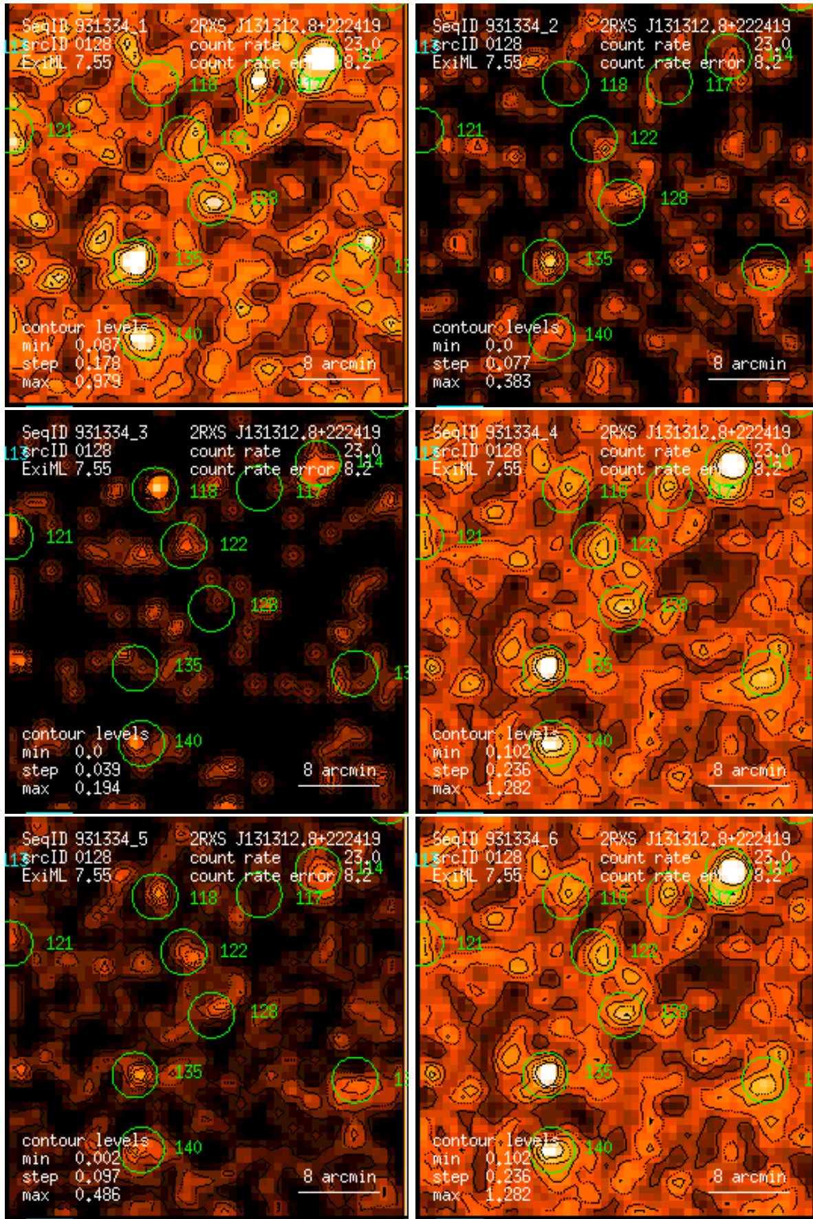
Figure 128: RASS 931334: detection 0128: band rate images, Gaussian filter: (1) PSPC channels 11 – 41, (2) 52 – 90, (3) 91 – 201, (4) 11 – 235, (5) 52 – 201, (6) 11 – 201. Broad band rates in counts/ks. Band rate contour levels in counts/ks/arcmin 2 .
