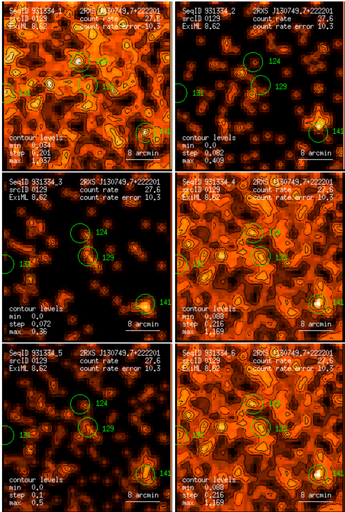
Figure 129: RASS 931334: detection 0129: band rate images, Gaussian filter: (1) PSPC channels 11 – 41, (2) 52 – 90, (3) 91 – 201, (4) 11 – 235, (5) 52 – 201, (6) 11 – 201. Broad band rates in counts/ks. Band rate contour levels in counts/ks/arcmin 2 .
