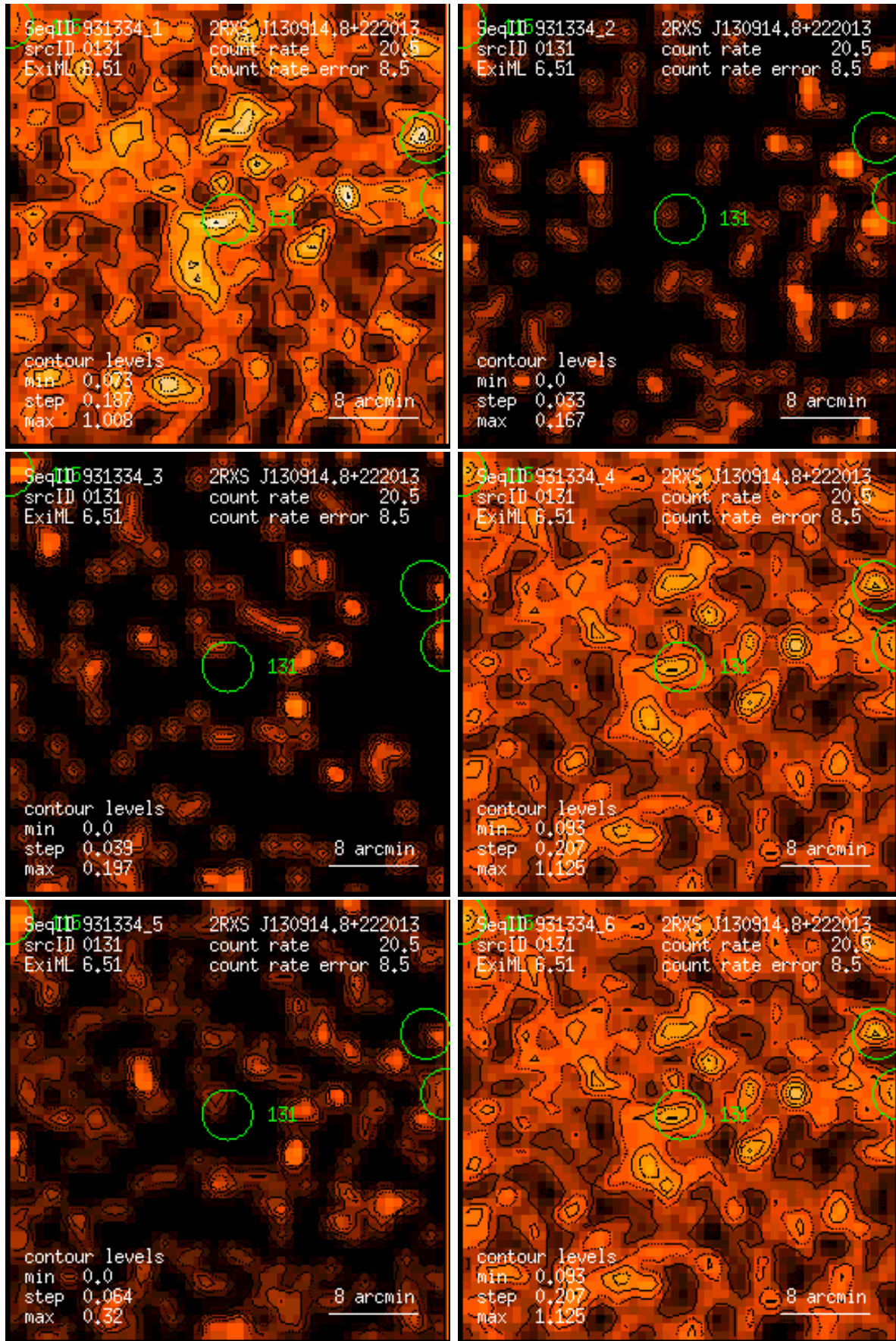
Figure 131: RASS 931334: detection 0131: band rate images, Gaussian filter: (1) PSPC channels 11 – 41, (2) 52 – 90, (3) 91 – 201, (4) 11 – 235, (5) 52 – 201, (6) 11 – 201. Broad band rates in counts/ks. Band rate contour levels in counts/ks/arcmin 2 .
