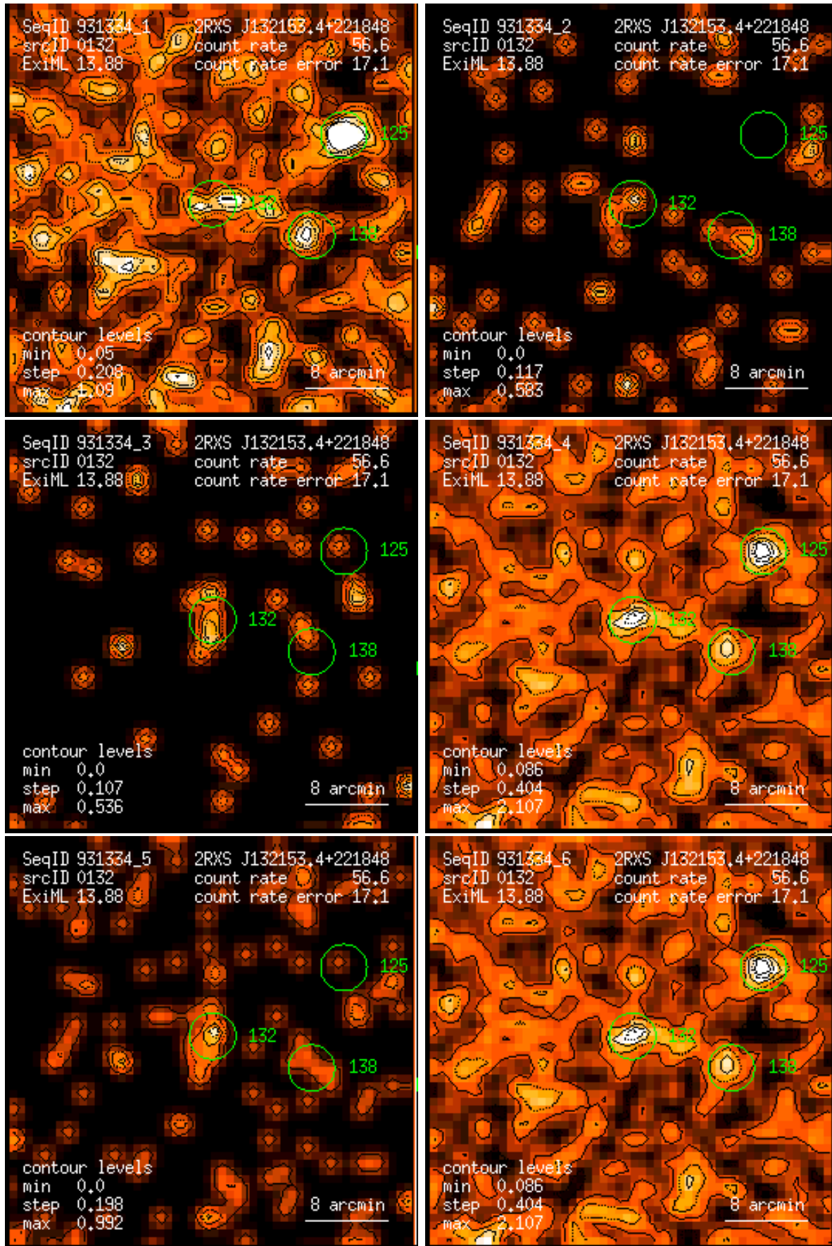
Figure 132: RASS 931334: detection 0132: band rate images, Gaussian filter: (1) PSPC channels 11 – 41, (2) 52 – 90, (3) 91 – 201, (4) 11 – 235, (5) 52 – 201, (6) 11 – 201. Broad band rates in counts/ks. Band rate contour levels in counts/ks/arcmin 2 .
