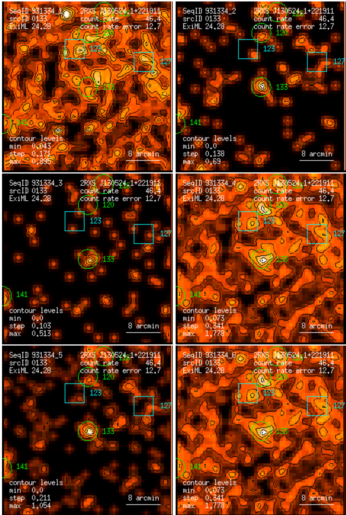
Figure 133: RASS 931334: detection 0133: band rate images, Gaussian filter: (1) PSPC channels 11 – 41, (2) 52 – 90, (3) 91 – 201, (4) 11 – 235, (5) 52 – 201, (6) 11 – 201. Broad band rates in counts/ks. Band rate contour levels in counts/ks/arcmin 2 .
