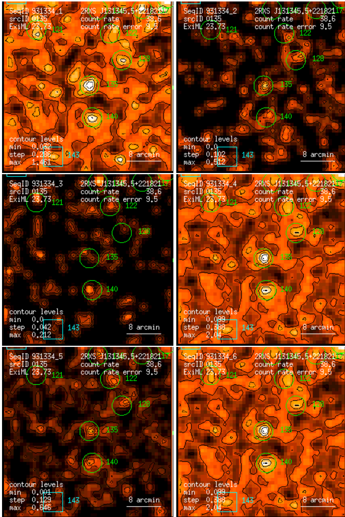
Figure 135: RASS 931334: detection 0135: band rate images, Gaussian filter: (1) PSPC channels 11 – 41, (2) 52 – 90, (3) 91 – 201, (4) 11 – 235, (5) 52 – 201, (6) 11 – 201. Broad band rates in counts/ks. Band rate contour levels in counts/ks/arcmin 2 .
