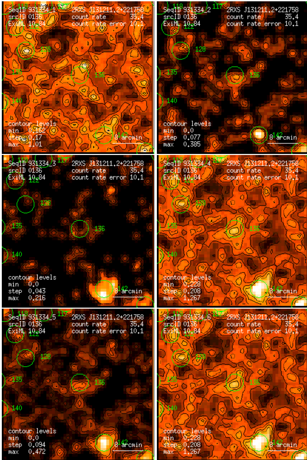
Figure 136: RASS 931334: detection 0136: band rate images, Gaussian filter: (1) PSPC channels 11 – 41, (2) 52 – 90, (3) 91 – 201, (4) 11 – 235, (5) 52 – 201, (6) 11 – 201. Broad band rates in counts/ks. Band rate contour levels in counts/ks/arcmin 2 .
