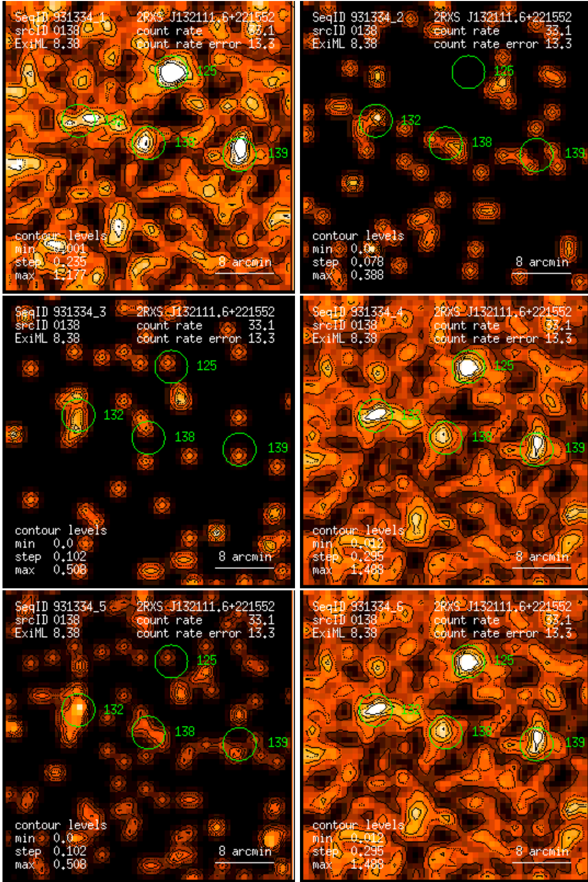
Figure 138: RASS 931334: detection 0138: band rate images, Gaussian filter: (1) PSPC channels 11 – 41, (2) 52 – 90, (3) 91 – 201, (4) 11 – 235, (5) 52 – 201, (6) 11 – 201. Broad band rates in counts/ks. Band rate contour levels in counts/ks/arcmin 2 .
