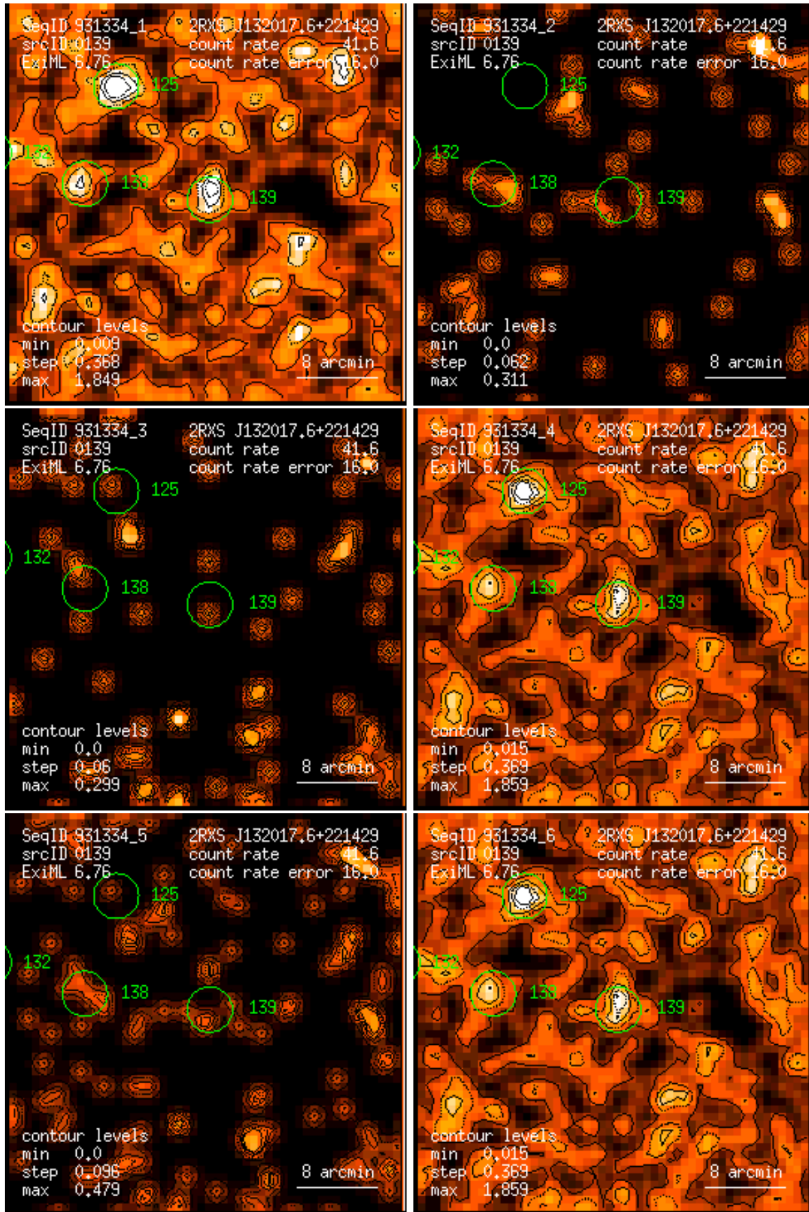
Figure 139: RASS 931334: detection 0139: band rate images, Gaussian filter: (1) PSPC channels 11 – 41, (2) 52 – 90, (3) 91 – 201, (4) 11 – 235, (5) 52 – 201, (6) 11 – 201. Broad band rates in counts/ks. Band rate contour levels in counts/ks/arcmin 2 .
