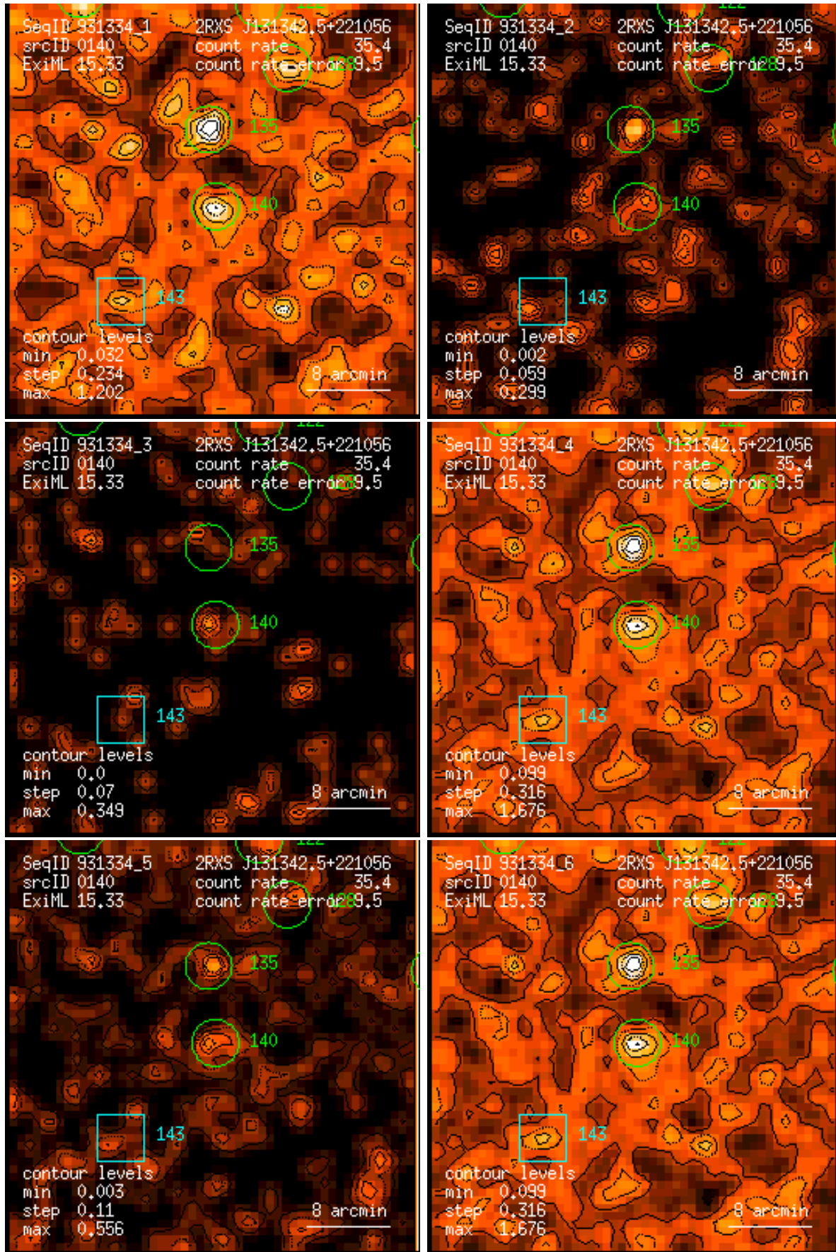
Figure 140: RASS 931334: detection 0140: band rate images, Gaussian filter: (1) PSPC channels 11 – 41, (2) 52 – 90, (3) 91 – 201, (4) 11 – 235, (5) 52 – 201, (6) 11 – 201. Broad band rates in counts/ks. Band rate contour levels in counts/ks/arcmin 2 .
