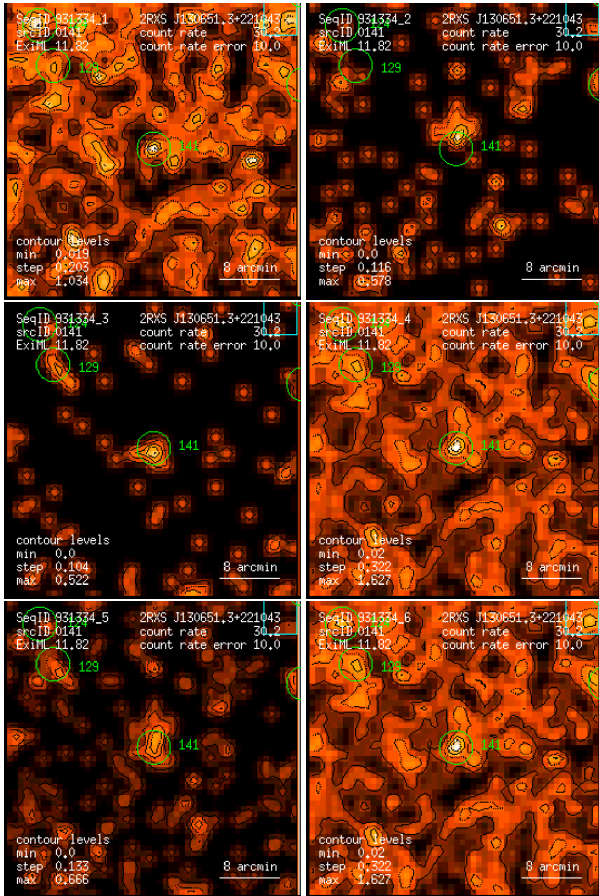
Figure 141: RASS 931334: detection 0141: band rate images, Gaussian filter: (1) PSPC channels 11 – 41, (2) 52 – 90, (3) 91 – 201, (4) 11 – 235, (5) 52 – 201, (6) 11 – 201. Broad band rates in counts/ks. Band rate contour levels in counts/ks/arcmin 2 .
