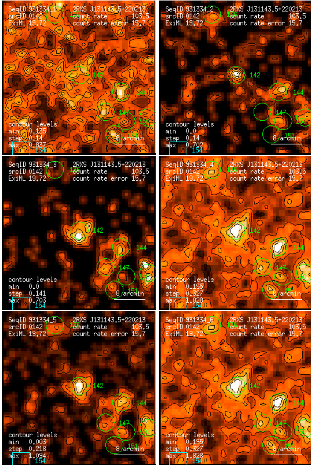
Figure 142: RASS 931334: detection 0142: band rate images, Gaussian filter: (1) PSPC channels 11 – 41, (2) 52 – 90, (3) 91 – 201, (4) 11 – 235, (5) 52 – 201, (6) 11 – 201. Broad band rates in counts/ks. Band rate contour levels in counts/ks/arcmin 2 .
