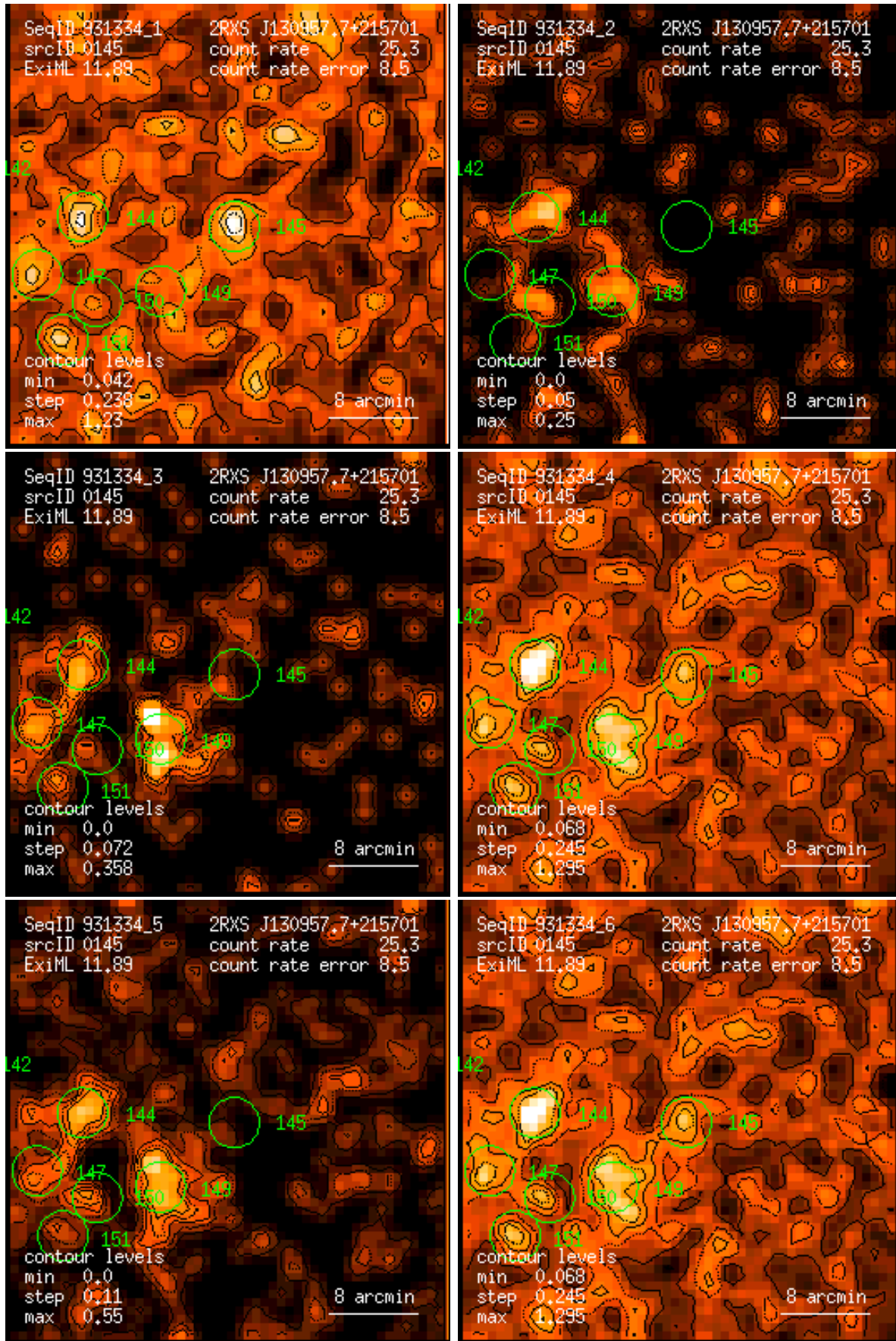
Figure 145: RASS 931334: detection 0145: band rate images, Gaussian filter: (1) PSPC channels 11 – 41, (2) 52 – 90, (3) 91 – 201, (4) 11 – 235, (5) 52 – 201, (6) 11 – 201. Broad band rates in counts/ks. Band rate contour levels in counts/ks/arcmin 2 .
