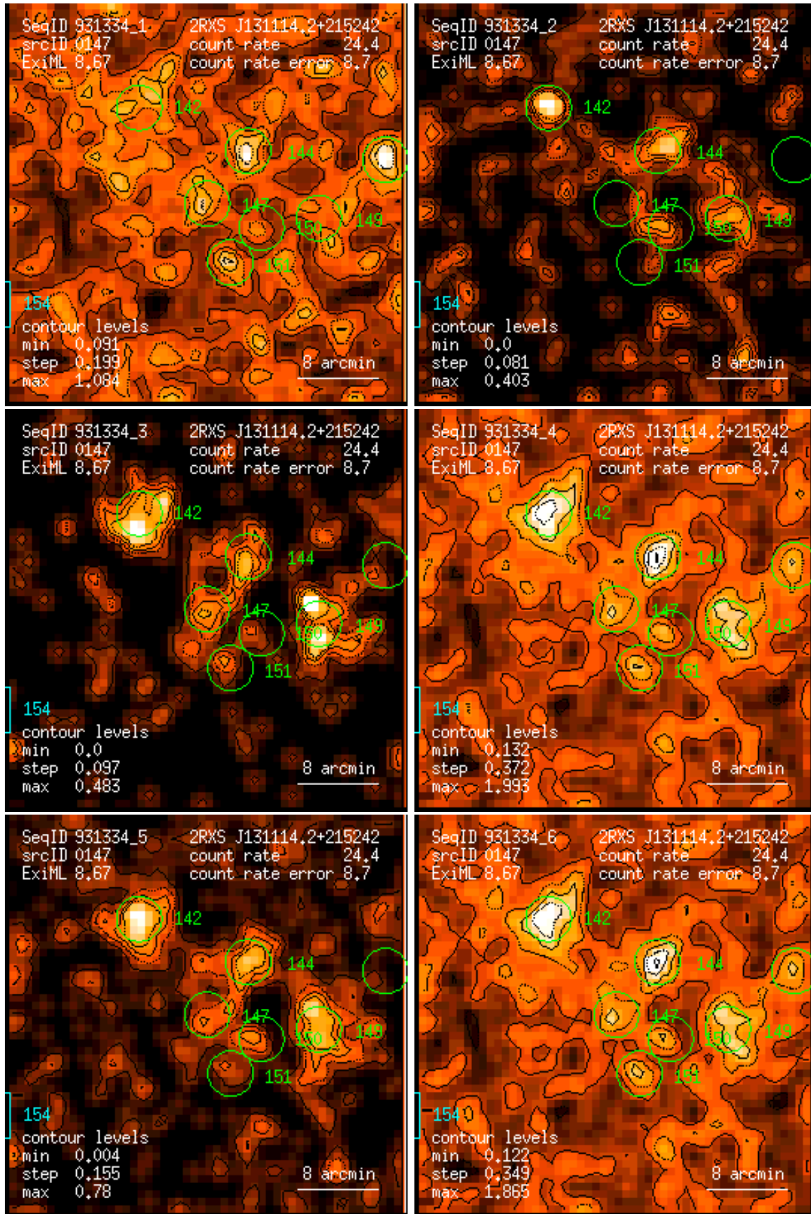
Figure 147: RASS 931334: detection 0147: band rate images, Gaussian filter: (1) PSPC channels 11 – 41, (2) 52 – 90, (3) 91 – 201, (4) 11 – 235, (5) 52 – 201, (6) 11 – 201. Broad band rates in counts/ks. Band rate contour levels in counts/ks/arcmin 2 .
