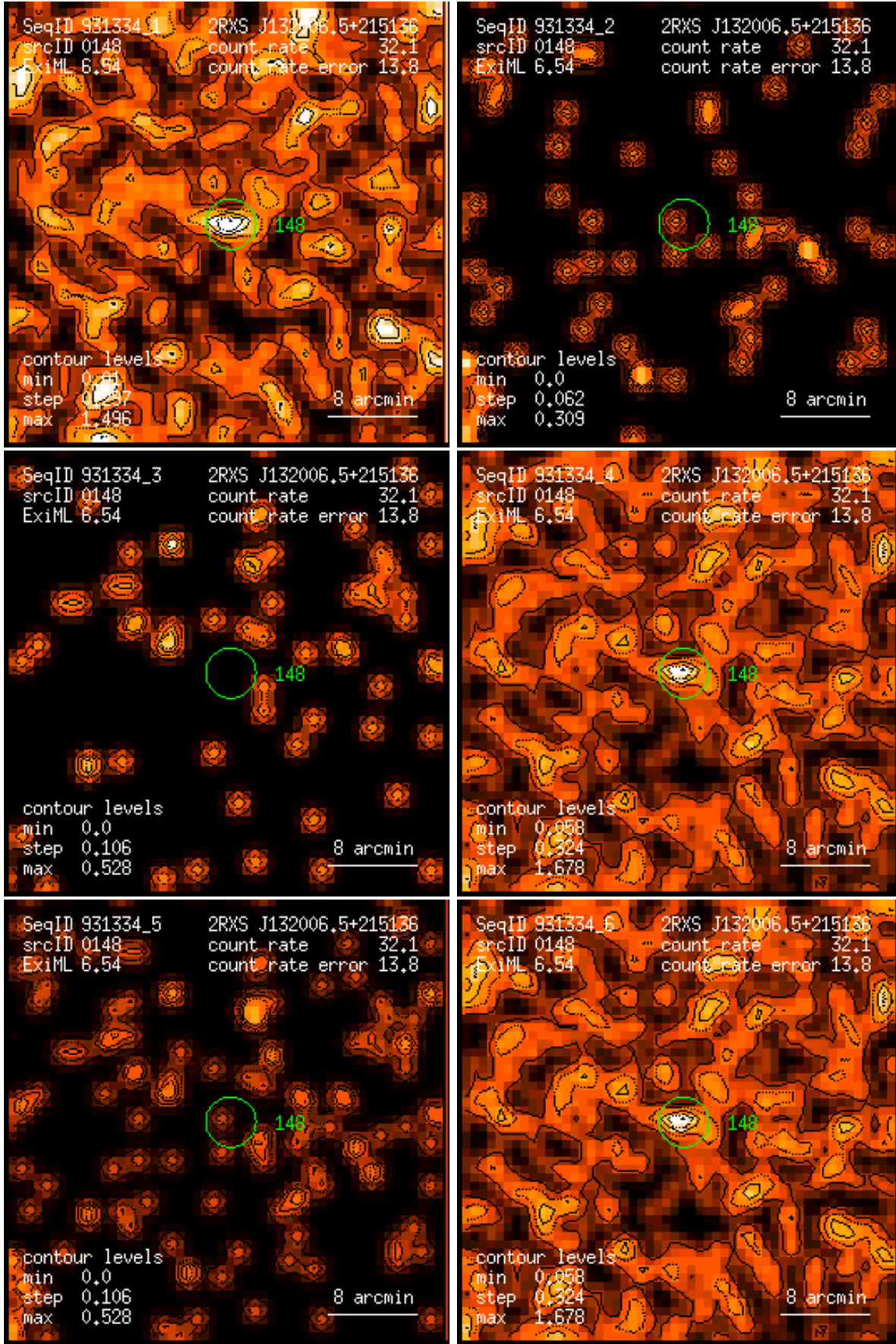
Figure 148: RASS 931334: detection 0148: band rate images, Gaussian filter: (1) PSPC channels 11 – 41, (2) 52 – 90, (3) 91 – 201, (4) 11 – 235, (5) 52 – 201, (6) 11 – 201. Broad band rates in counts/ks. Band rate contour levels in counts/ks/arcmin 2 .
