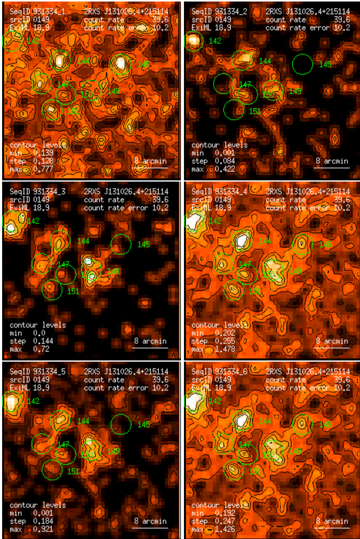
Figure 149: RASS 931334: detection 0149: band rate images, Gaussian filter: (1) PSPC channels 11 – 41, (2) 52 – 90, (3) 91 – 201, (4) 11 – 235, (5) 52 – 201, (6) 11 – 201. Broad band rates in counts/ks. Band rate contour levels in counts/ks/arcmin 2 .
