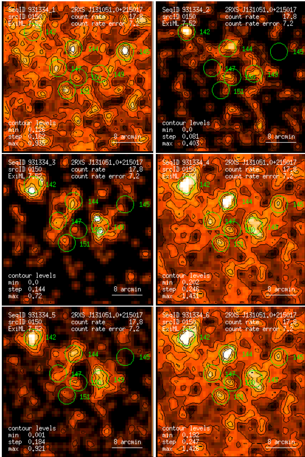
Figure 150: RASS 931334: detection 0150: band rate images, Gaussian filter: (1) PSPC channels 11 – 41, (2) 52 – 90, (3) 91 – 201, (4) 11 – 235, (5) 52 – 201, (6) 11 – 201. Broad band rates in counts/ks. Band rate contour levels in counts/ks/arcmin 2 .
