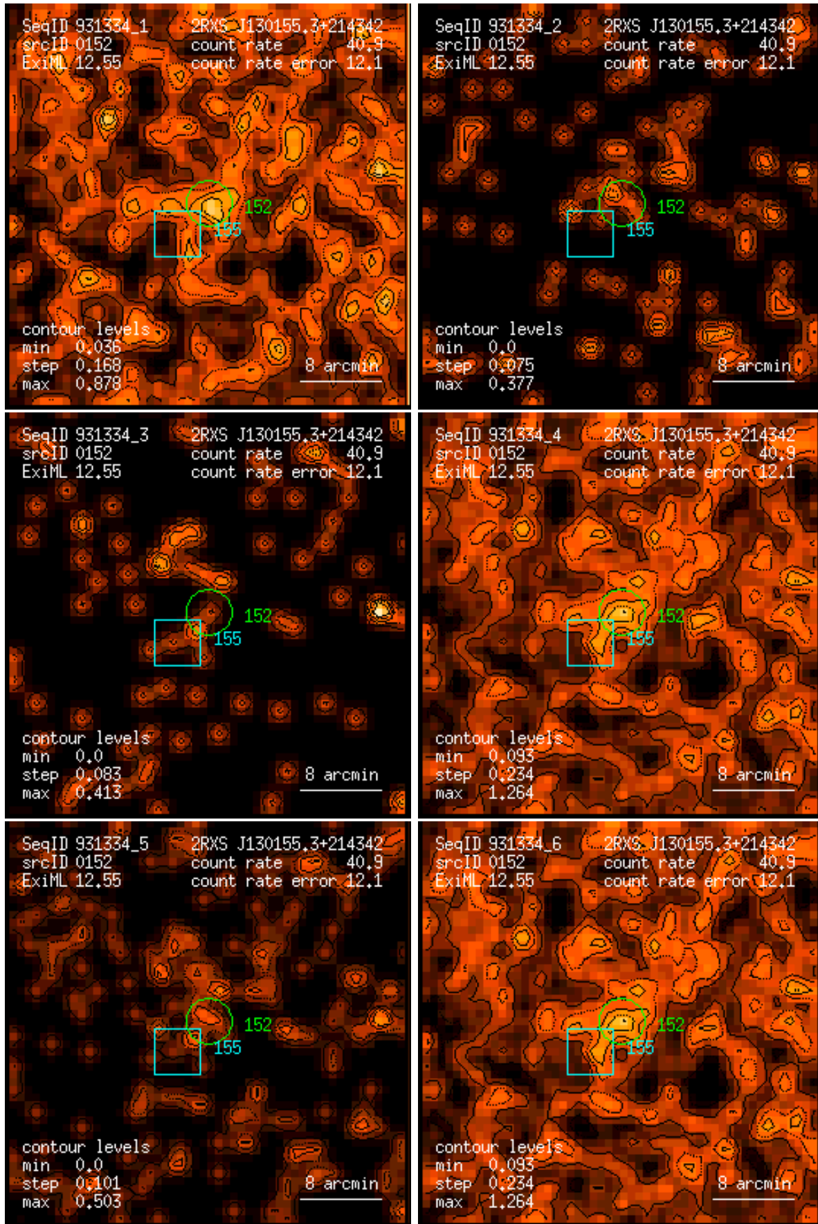
Figure 152: RASS 931334: detection 0152: band rate images, Gaussian filter: (1) PSPC channels 11 – 41, (2) 52 – 90, (3) 91 – 201, (4) 11 – 235, (5) 52 – 201, (6) 11 – 201. Broad band rates in counts/ks. Band rate contour levels in counts/ks/arcmin 2 .
