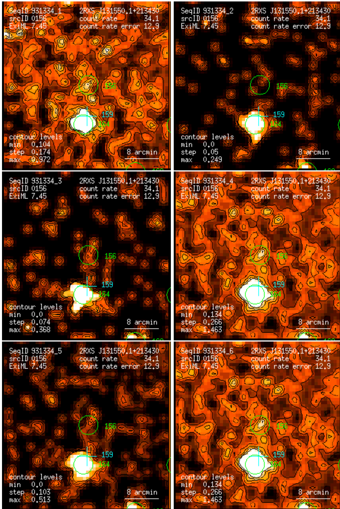
Figure 156: RASS 931334: detection 0156: band rate images, Gaussian filter: (1) PSPC channels 11 – 41, (2) 52 – 90, (3) 91 – 201, (4) 11 – 235, (5) 52 – 201, (6) 11 – 201. Broad band rates in counts/ks. Band rate contour levels in counts/ks/arcmin 2 .
