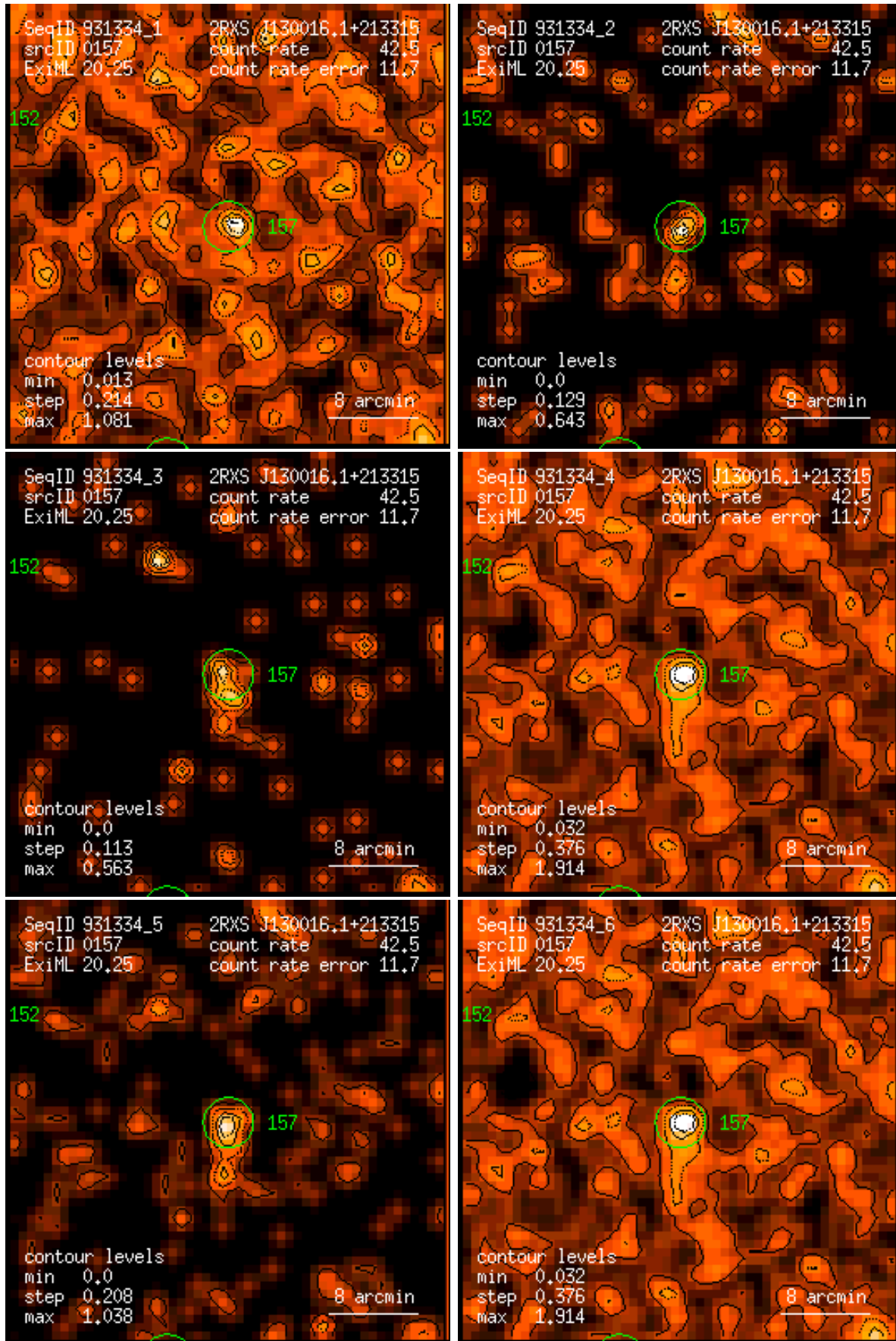
Figure 157: RASS 931334: detection 0157: band rate images, Gaussian filter: (1) PSPC channels 11 – 41, (2) 52 – 90, (3) 91 – 201, (4) 11 – 235, (5) 52 – 201, (6) 11 – 201. Broad band rates in counts/ks. Band rate contour levels in counts/ks/arcmin 2 .
