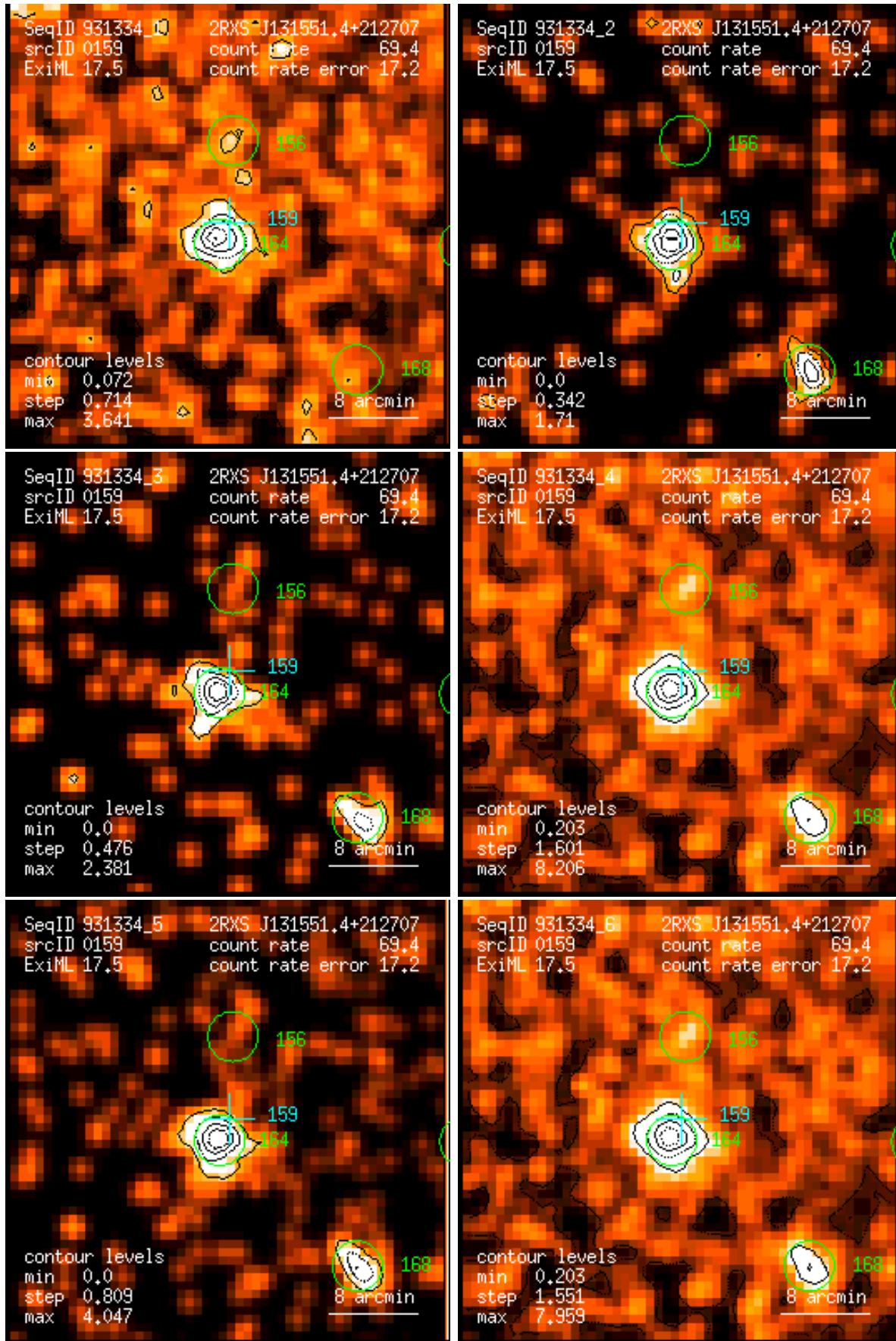
Figure 159: RASS 931334: detection 0159: band rate images, Gaussian filter: (1) PSPC channels 11 – 41, (2) 52 – 90, (3) 91 – 201, (4) 11 – 235, (5) 52 – 201, (6) 11 – 201. Broad band rates in counts/ks. Band rate contour levels in counts/ks/arcmin 2 .
