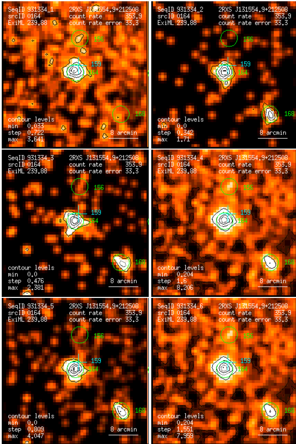
Figure 164: RASS 931334: detection 0164: band rate images, Gaussian filter: (1) PSPC channels 11 – 41, (2) 52 – 90, (3) 91 – 201, (4) 11 – 235, (5) 52 – 201, (6) 11 – 201. Broad band rates in counts/ks. Band rate contour levels in counts/ks/arcmin 2 .
