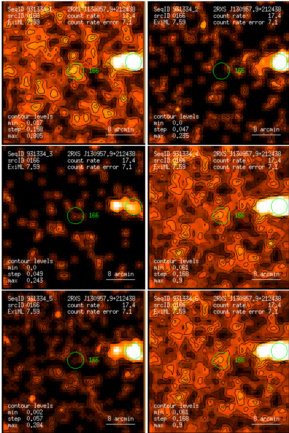
Figure 166: RASS 931334: detection 0166: band rate images, Gaussian filter: (1) PSPC channels 11 – 41, (2) 52 – 90, (3) 91 – 201, (4) 11 – 235, (5) 52 – 201, (6) 11 – 201. Broad band rates in counts/ks. Band rate contour levels in counts/ks/arcmin 2 .
