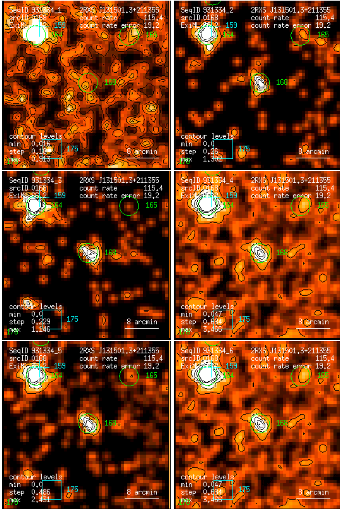
Figure 168: RASS 931334: detection 0168: band rate images, Gaussian filter: (1) PSPC channels 11 – 41, (2) 52 – 90, (3) 91 – 201, (4) 11 – 235, (5) 52 – 201, (6) 11 – 201. Broad band rates in counts/ks. Band rate contour levels in counts/ks/arcmin 2 .
