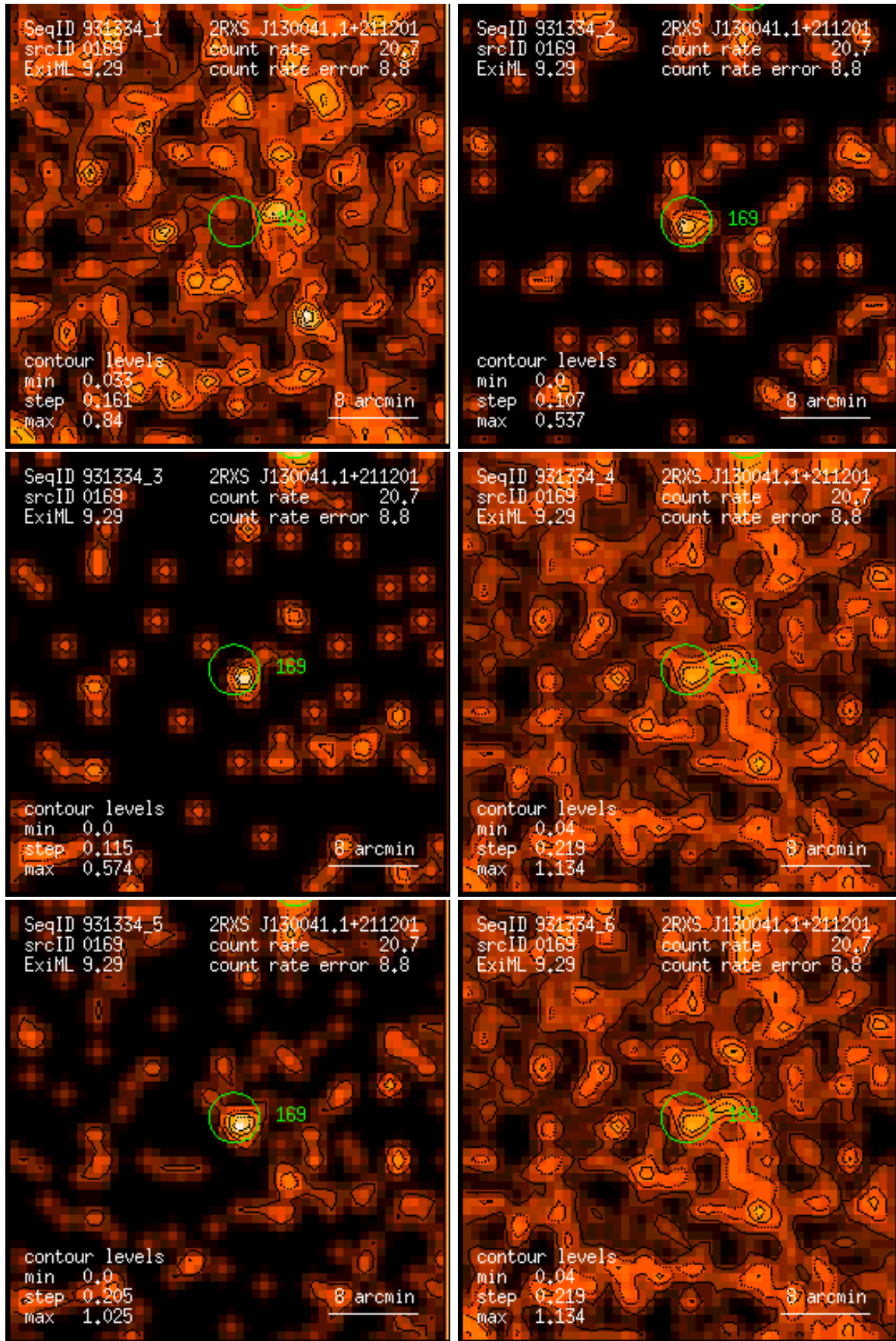
Figure 169: RASS 931334: detection 0169: band rate images, Gaussian filter: (1) PSPC channels 11 – 41, (2) 52 – 90, (3) 91 – 201, (4) 11 – 235, (5) 52 – 201, (6) 11 – 201. Broad band rates in counts/ks. Band rate contour levels in counts/ks/arcmin 2 .
