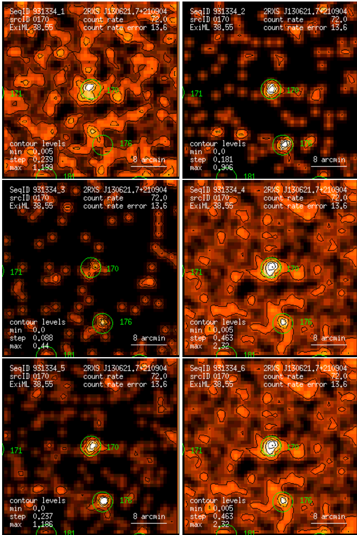
Figure 170: RASS 931334: detection 0170: band rate images, Gaussian filter: (1) PSPC channels 11 – 41, (2) 52 – 90, (3) 91 – 201, (4) 11 – 235, (5) 52 – 201, (6) 11 – 201. Broad band rates in counts/ks. Band rate contour levels in counts/ks/arcmin 2 .
