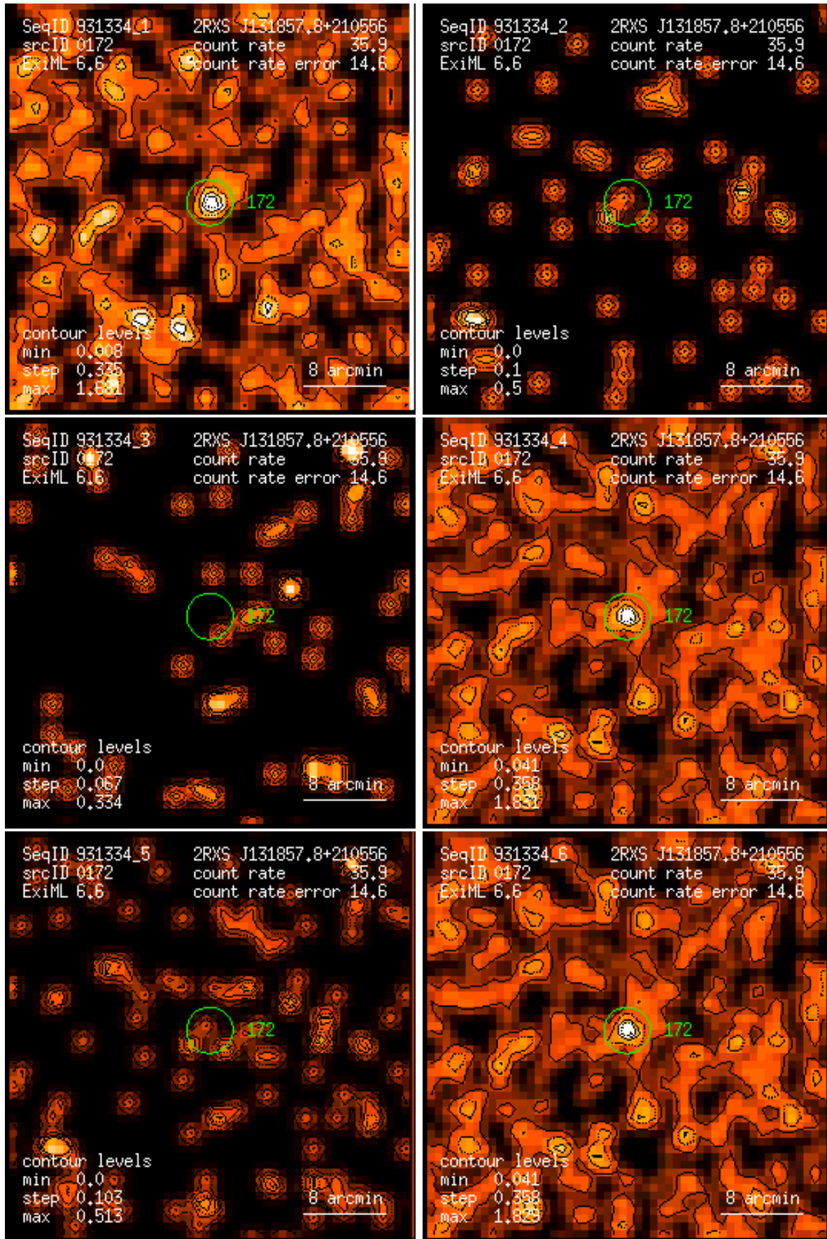
Figure 172: RASS 931334: detection 0172: band rate images, Gaussian filter: (1) PSPC channels 11 – 41, (2) 52 – 90, (3) 91 – 201, (4) 11 – 235, (5) 52 – 201, (6) 11 – 201. Broad band rates in counts/ks. Band rate contour levels in counts/ks/arcmin 2 .
