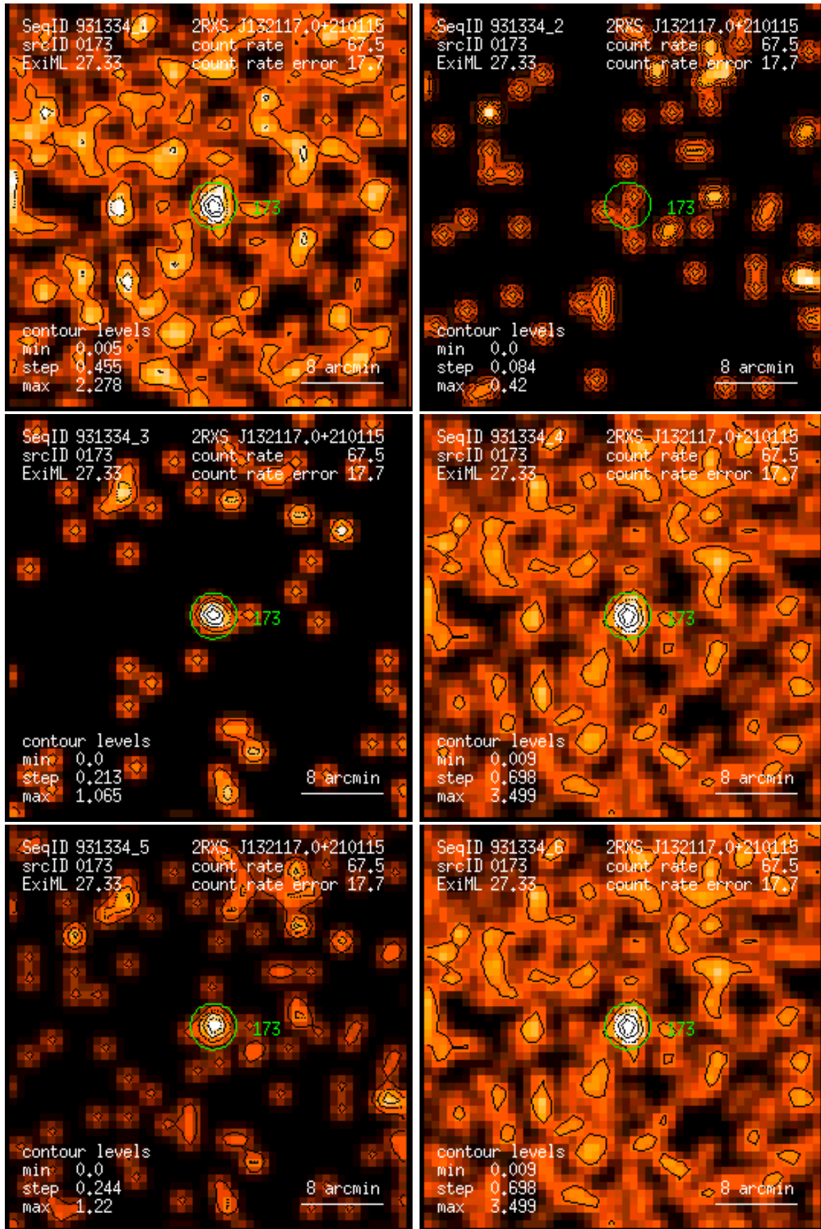
Figure 173: RASS 931334: detection 0173: band rate images, Gaussian filter: (1) PSPC channels 11 – 41, (2) 52 – 90, (3) 91 – 201, (4) 11 – 235, (5) 52 – 201, (6) 11 – 201. Broad band rates in counts/ks. Band rate contour levels in counts/ks/arcmin 2 .
