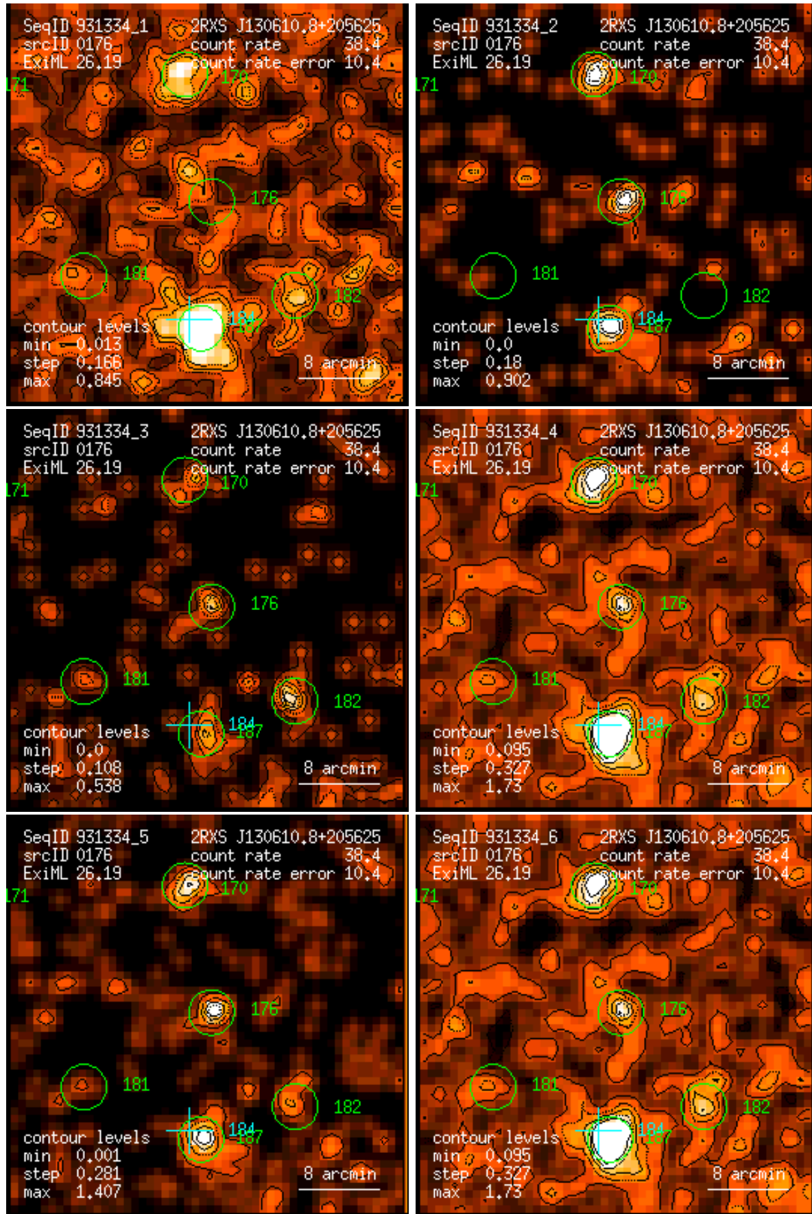
Figure 176: RASS 931334: detection 0176: band rate images, Gaussian filter: (1) PSPC channels 11 – 41, (2) 52 – 90, (3) 91 – 201, (4) 11 – 235, (5) 52 – 201, (6) 11 – 201. Broad band rates in counts/ks. Band rate contour levels in counts/ks/arcmin 2 .
