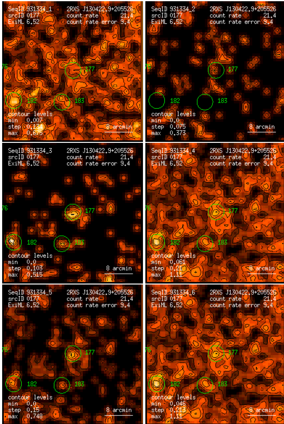
Figure 177: RASS 931334: detection 0177: band rate images, Gaussian filter: (1) PSPC channels 11 – 41, (2) 52 – 90, (3) 91 – 201, (4) 11 – 235, (5) 52 – 201, (6) 11 – 201. Broad band rates in counts/ks. Band rate contour levels in counts/ks/arcmin 2 .
